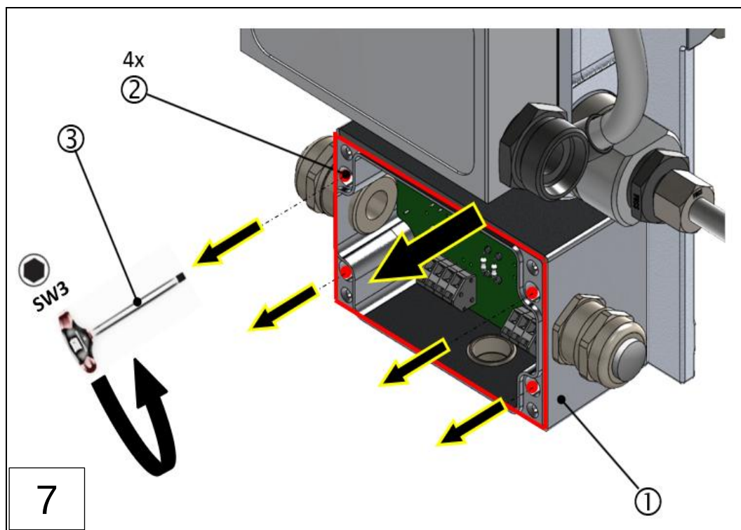
1: Klemmenkasten, VN2020 (alt)
