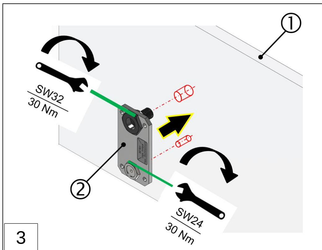
1: Motorwand
