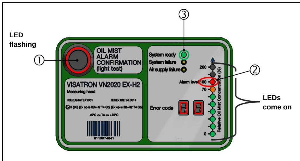
Fig.: 59 : VN2020 EX-H2 measuring head: "Alarm" status indicator at 100% OMC
