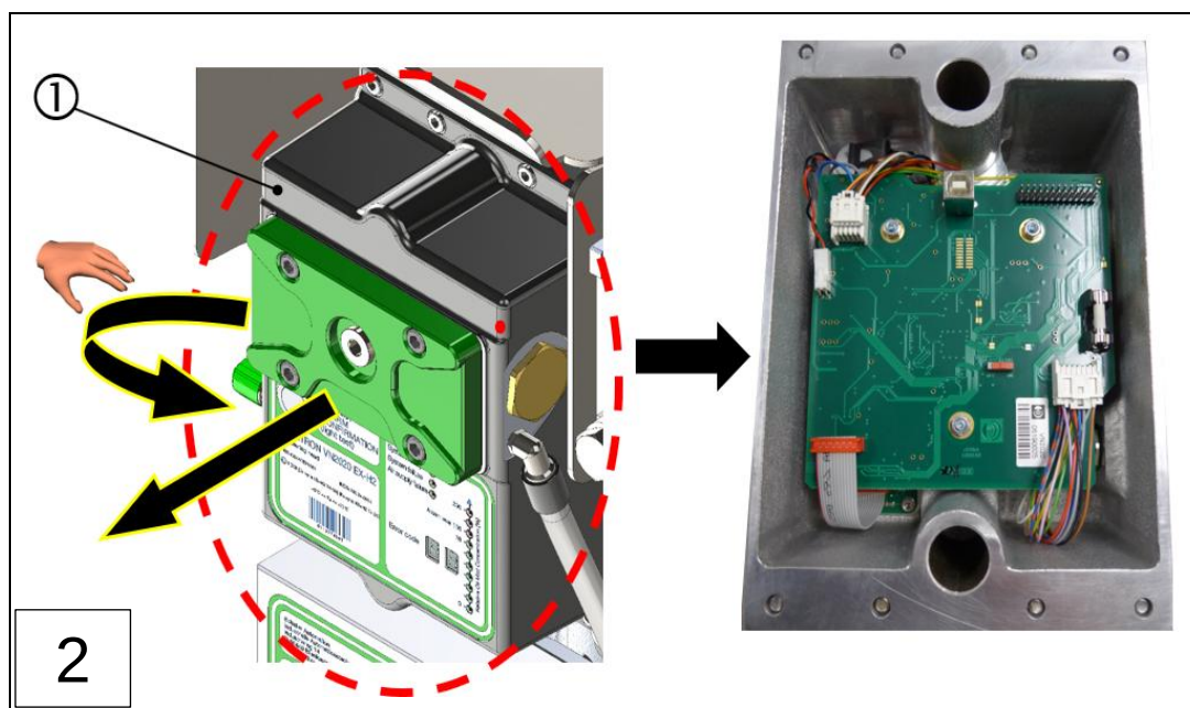
Fig.: 53 : Removing the VN2020 EX-H2 measuring head (installation steps 1-2)
