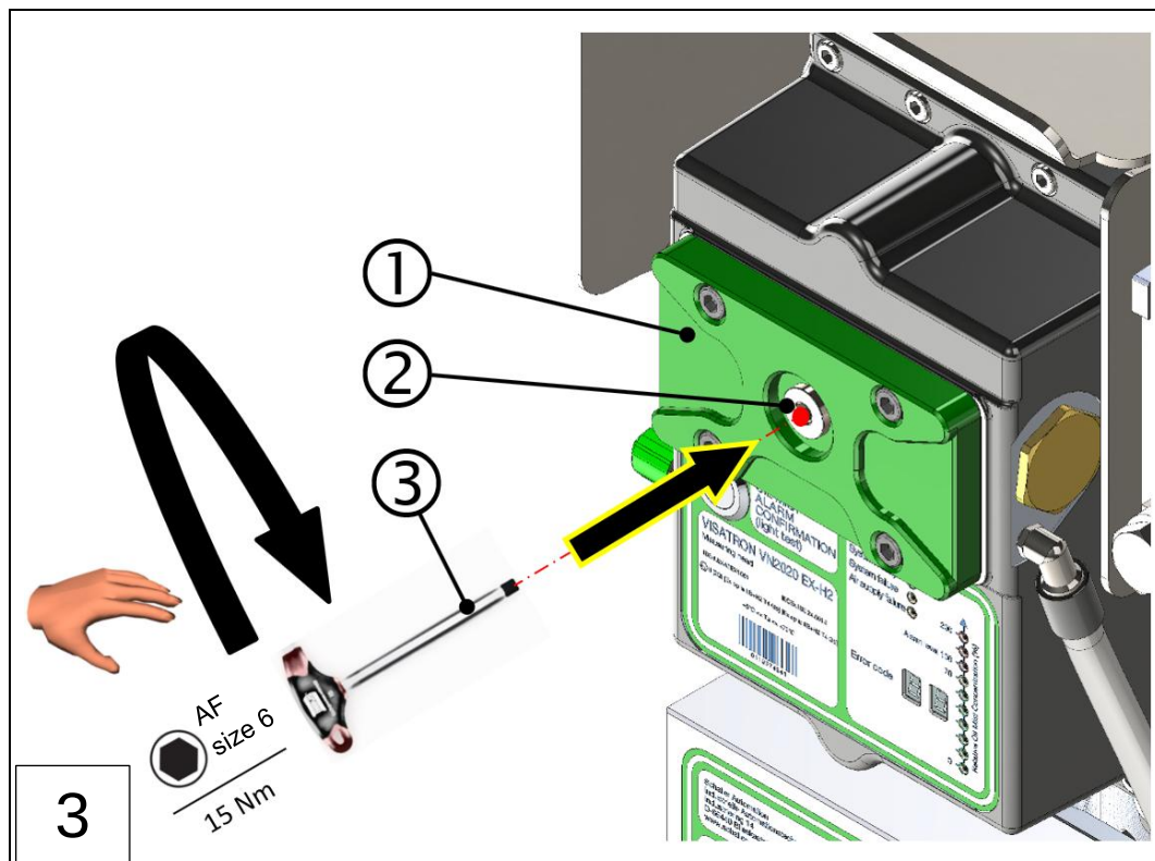
Fig.: 74 : Replacing the screw plug on the VN2020 EX-H2 measuring head (steps 1-3)
