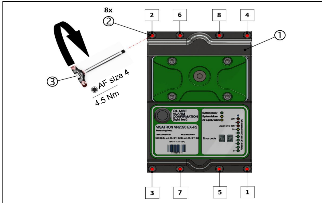
Fig.: 55 : Installing the VN2020 EX-H2 measuring head
