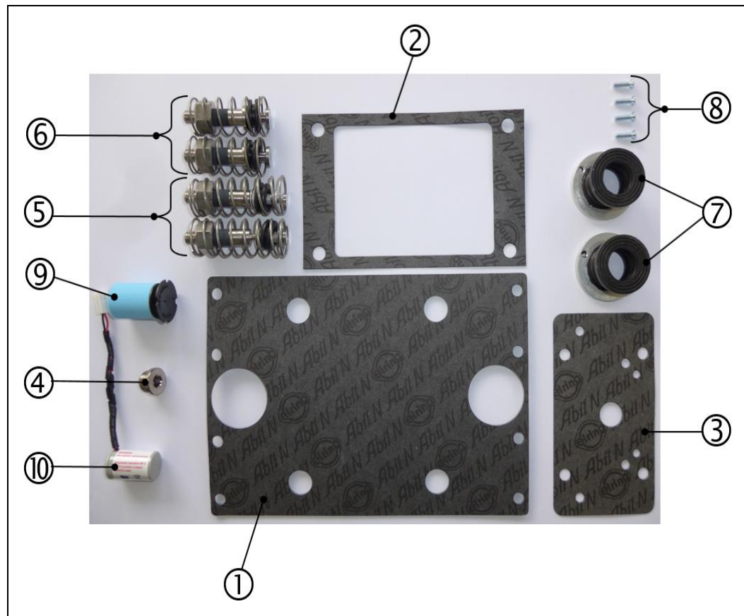
Fig.: 85 : Service kit for the VISATRON® VN2020 EX-H2
