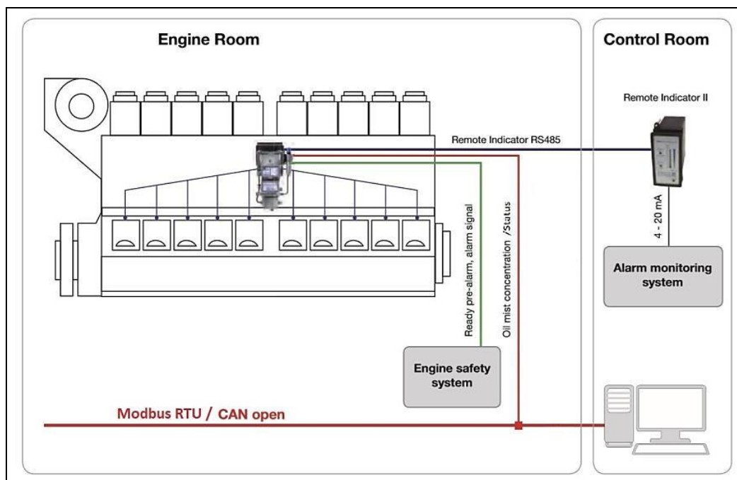
Fig.: 29 : Connection diagram for VN2020 series
