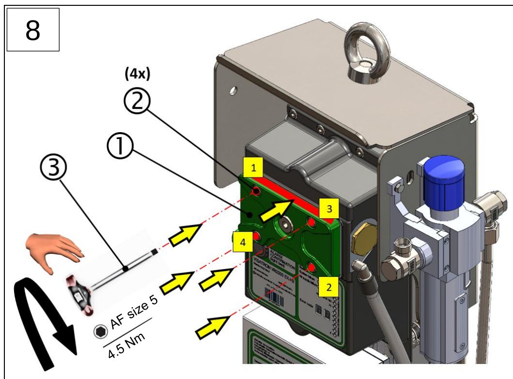
Fig.: 62 : Cleaning the light path of the VN2020 EX-H2 (steps 1-8)
