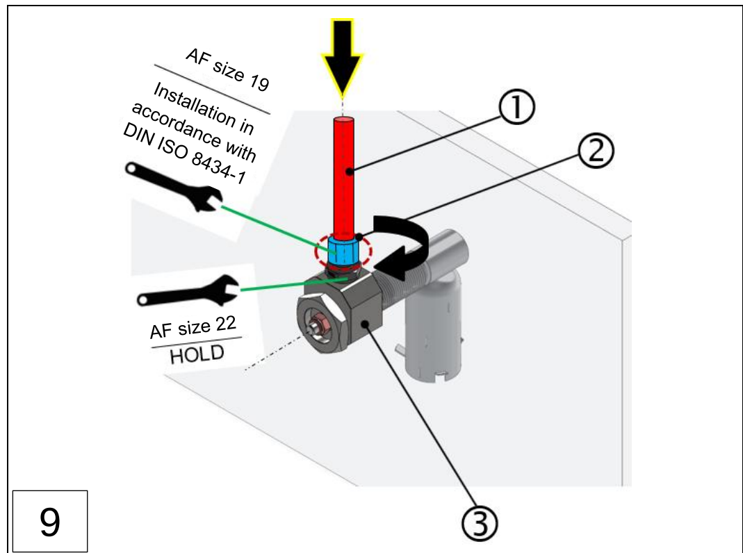
Fig.: 20 : Installing the engine wall connection for the VN2020 (installation steps 1-9)
