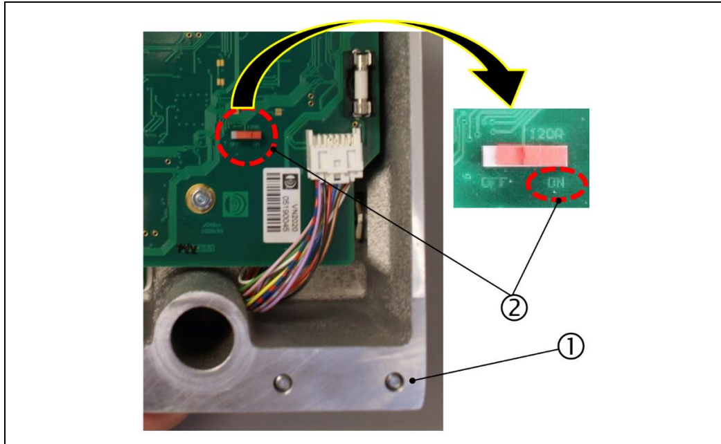
Fig.: 39 : Connection board for VN2020 EX-H2 measuring head
