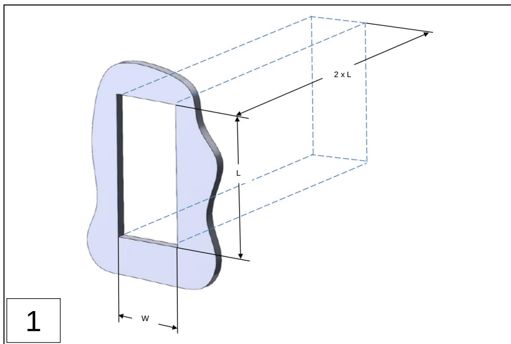
Fig.: 27 : Dimensions of installation space for Remote Indicator II
