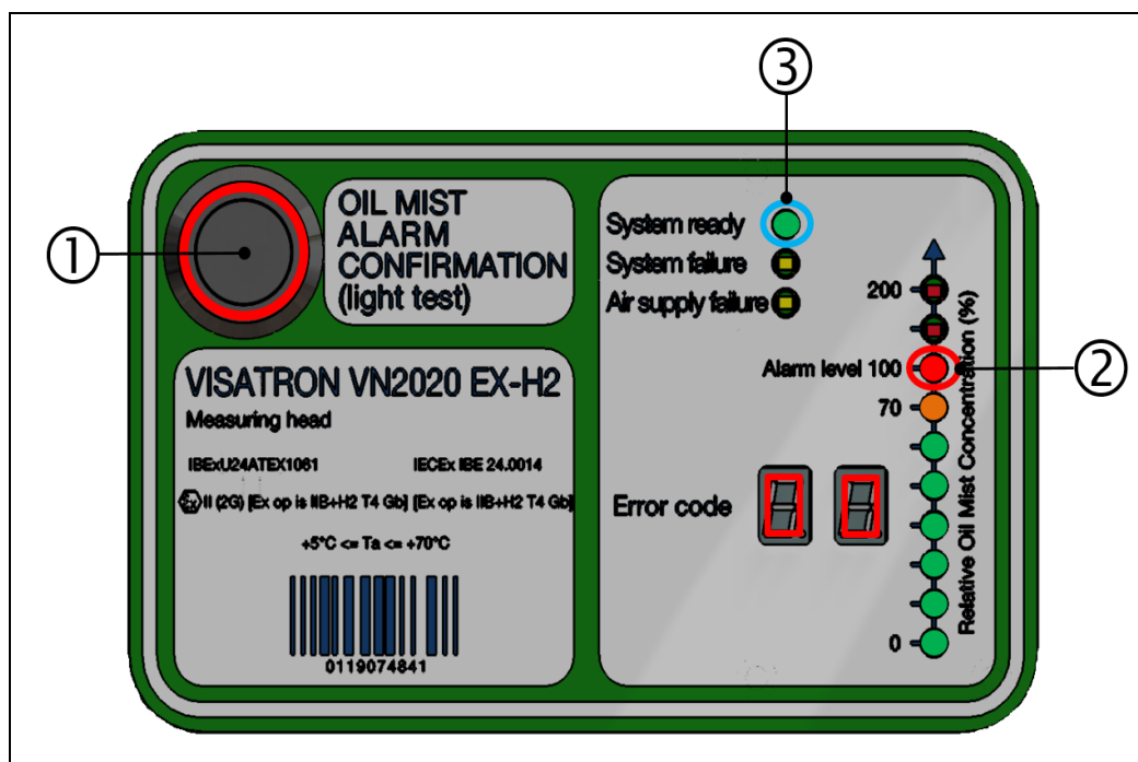
Fig.: 48 : Function test, starting up for the first time, VN2020 EX-H2
