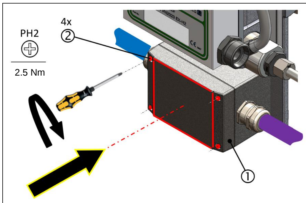
Fig.: 41 : Closing the terminal box for the VN2020 EX-H2
