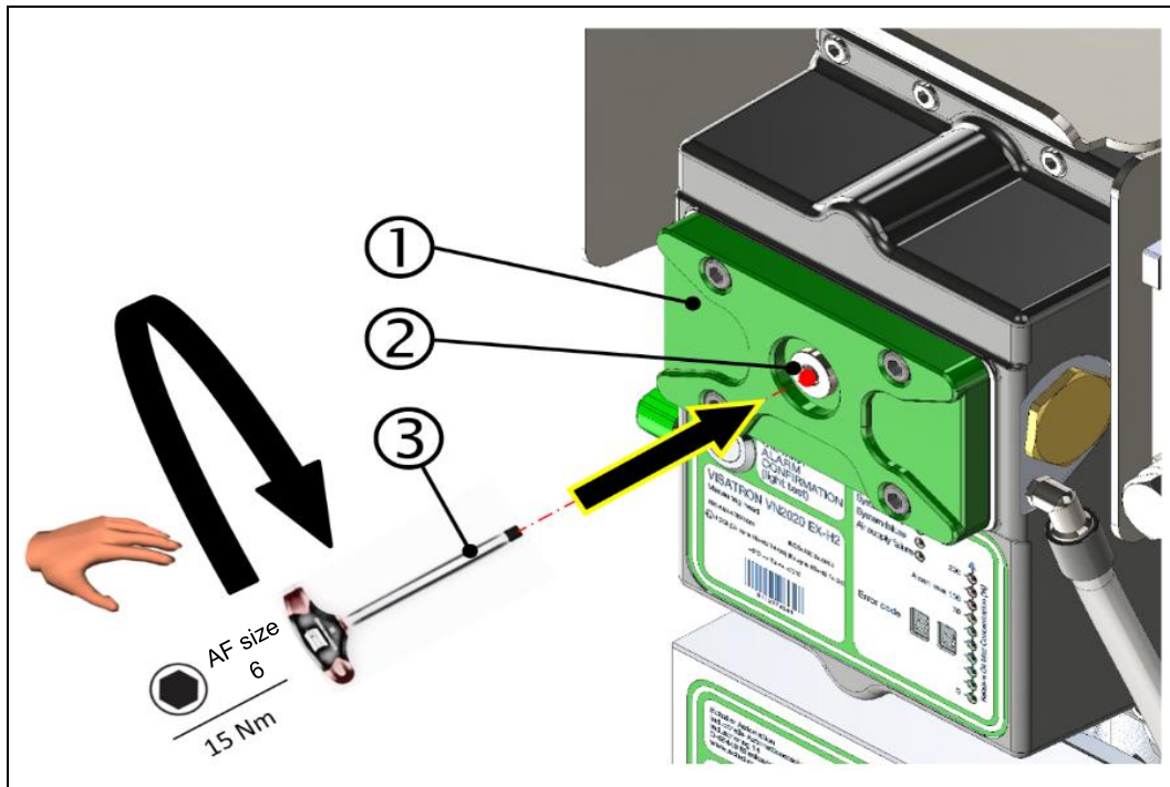
Fig.: 46 : Screwing in the screw plug on the measuring head of the VN2020 EX-H2
