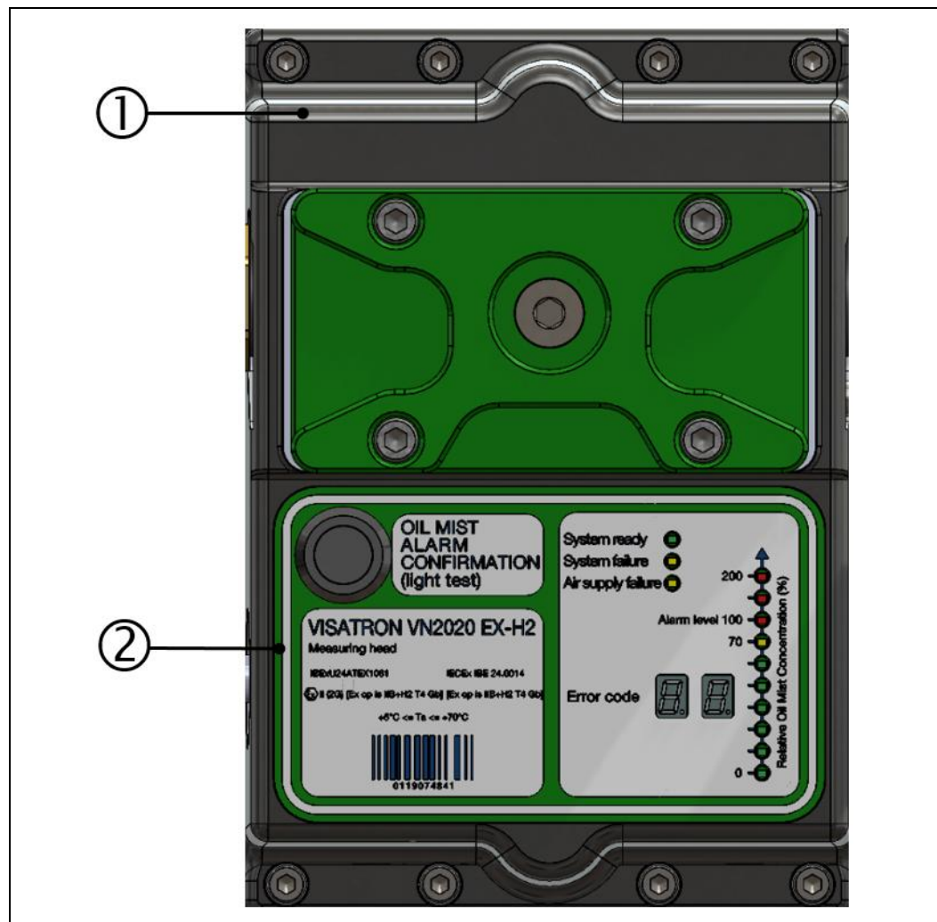
Fig.: 1 : VISATRON ® VN2020 EX-H2 measuring head
