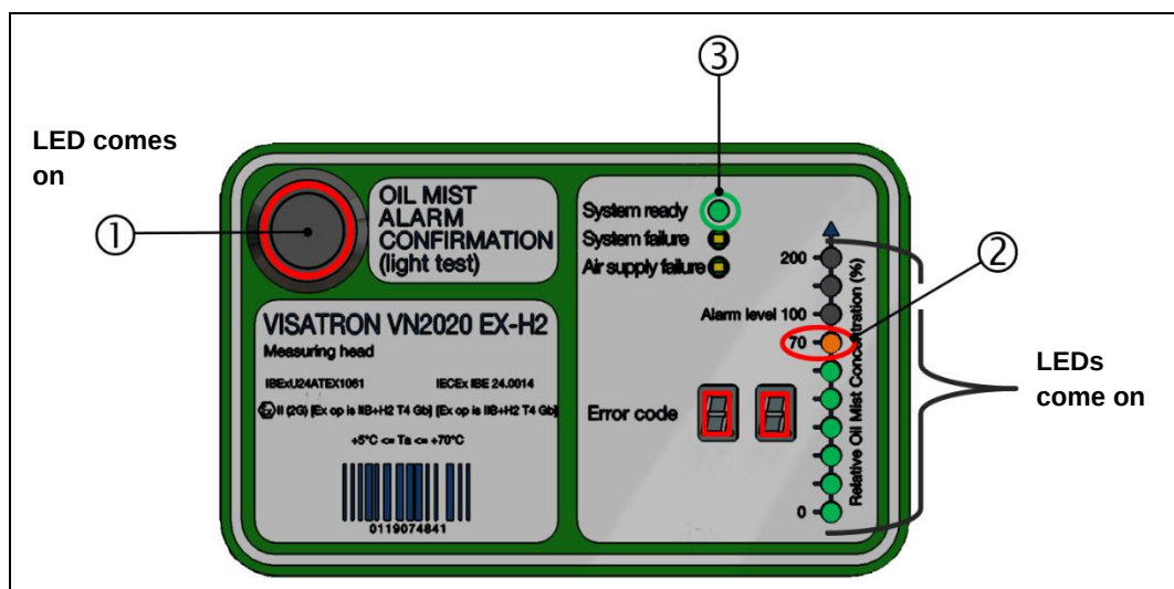
Fig.: 58 : VN2020 EX-H2 measuring head: “Pre-alarm” status indicator at 70% OMC
