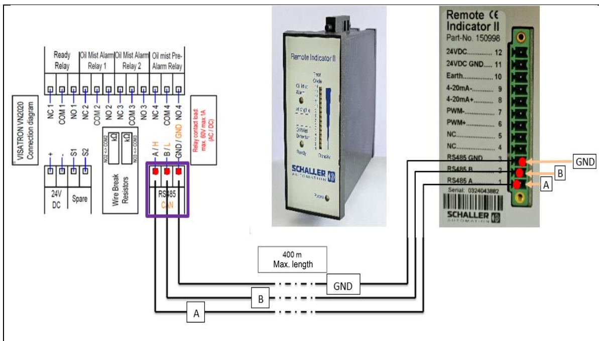
Fig.: 40 : Remote Indicator II (optional); installing contacts
