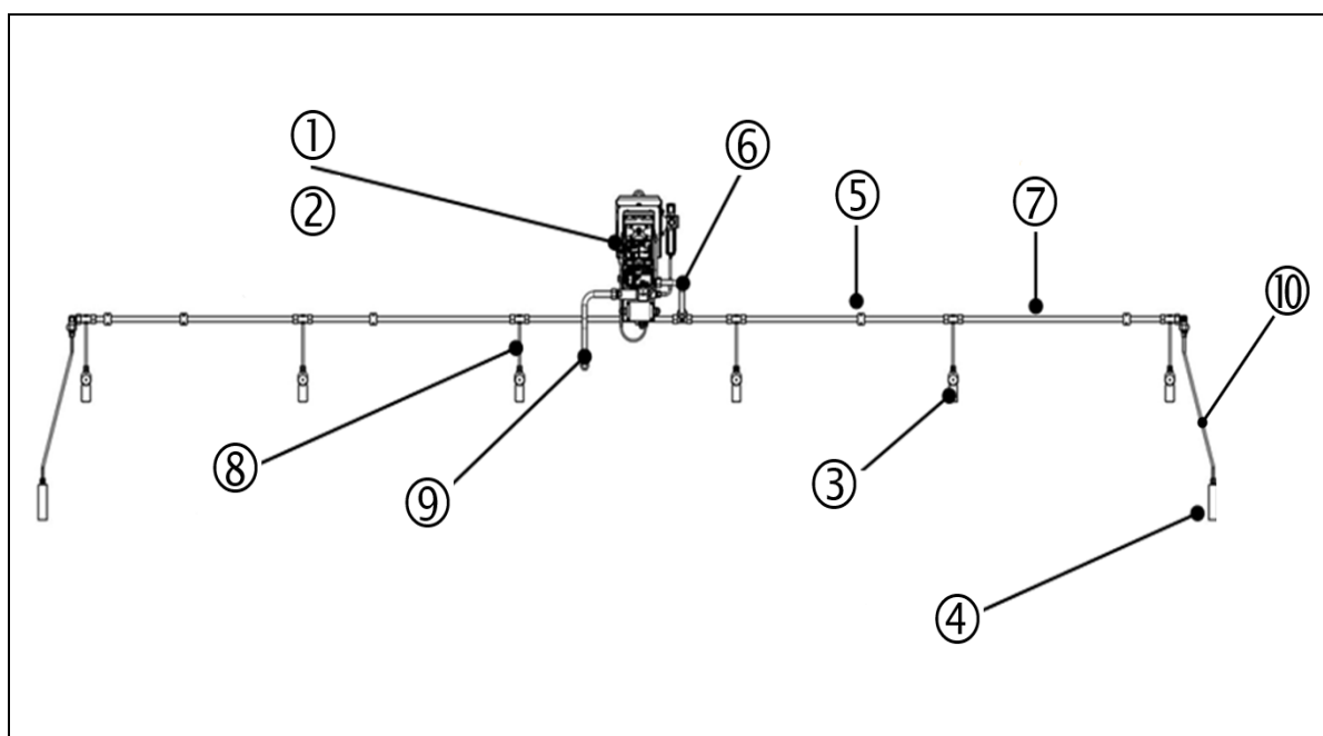
Fig.: 6 : Component overview, standard drainage, VISATRON® VN2020 EX-H2
