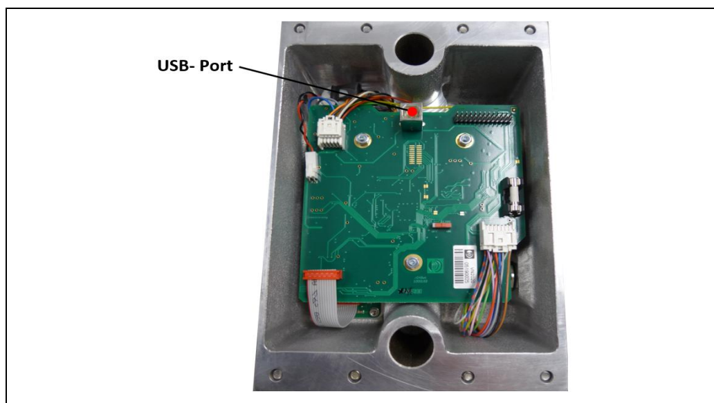
Fig.: 52 : Measuring head for VN2020 EX-H2, rear view, USB port
