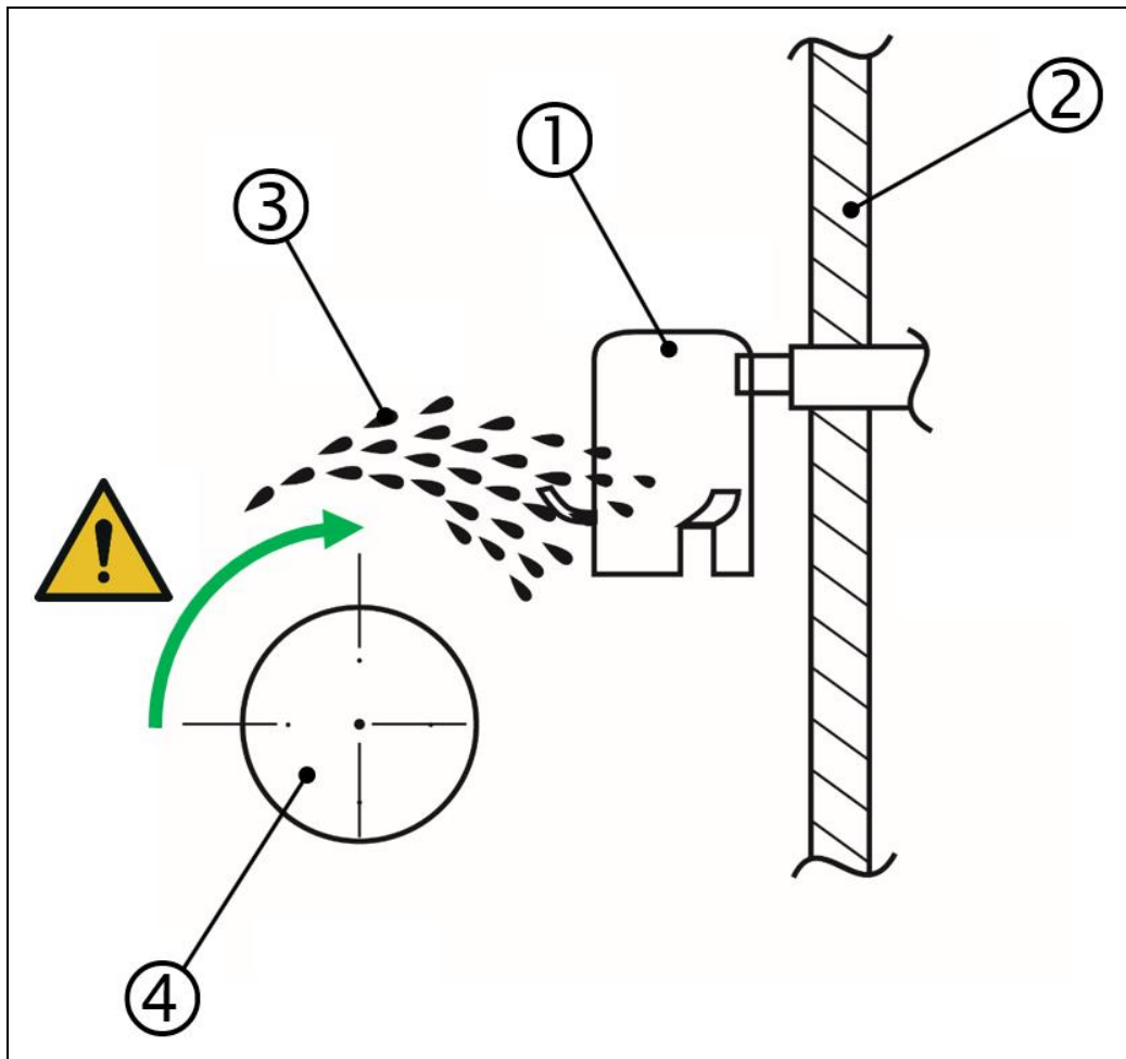
Fig.: 19 : Recommended inst. for the engine wall connection (view from the crankshaft end)
