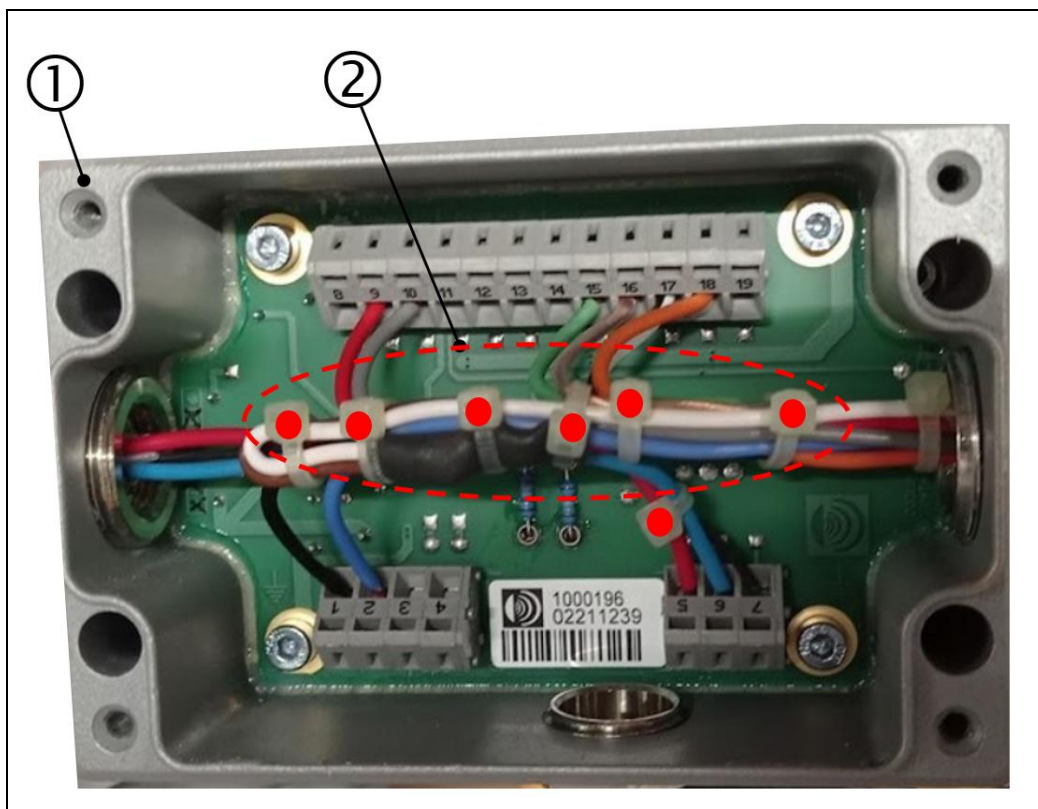
Fig.: 36 : Recommended electrical installation, terminal box for VN200 EX-H2
