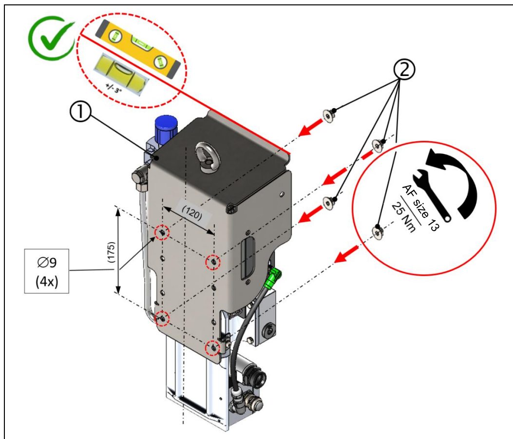
Fig.: 16 : Installing the VN2020 EX-H2 without bracket and with protective cover (rear view)
