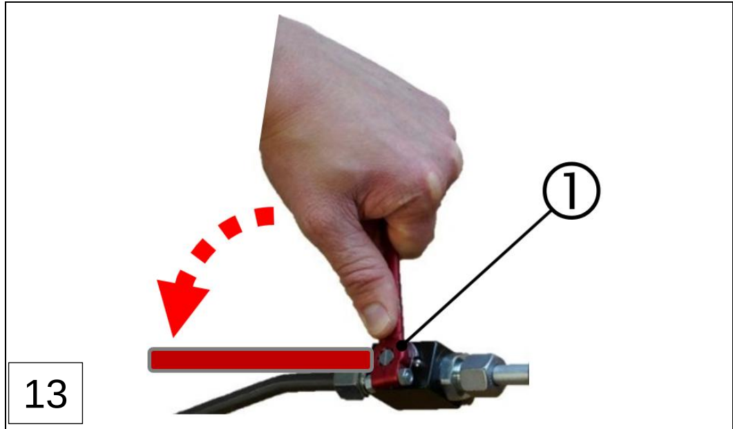
Fig.: 69 : Replacing the seal on the connecting box (steps 1- 13), VN2020 EX-H2
