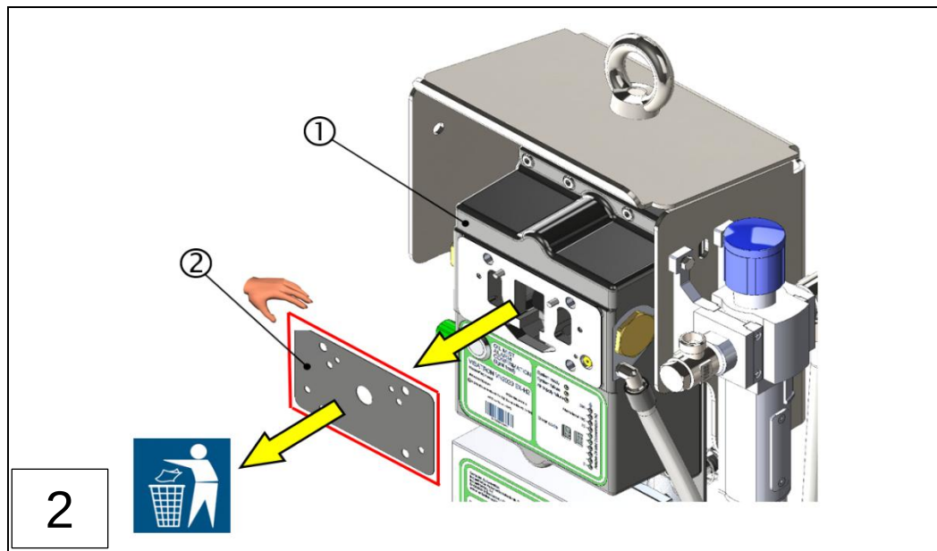
1: VN2020 EX-H2 measuring head
