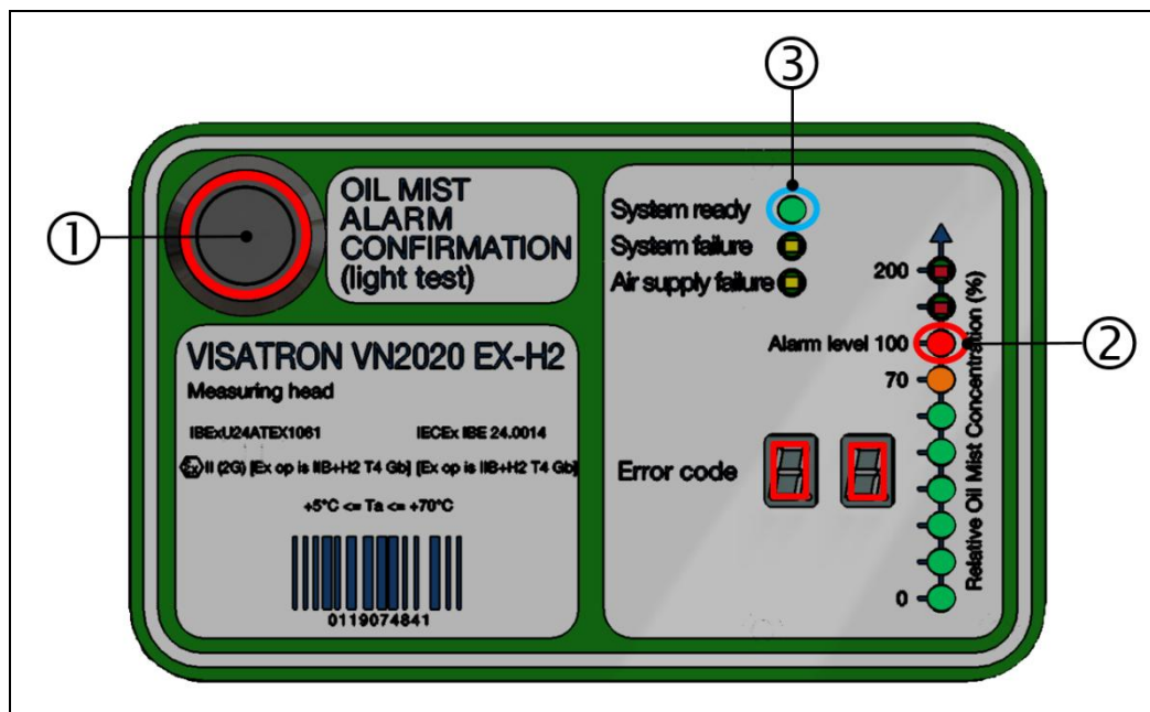
Fig.: 51 : Function test, starting up for the first time, VN2020 EX-H2
