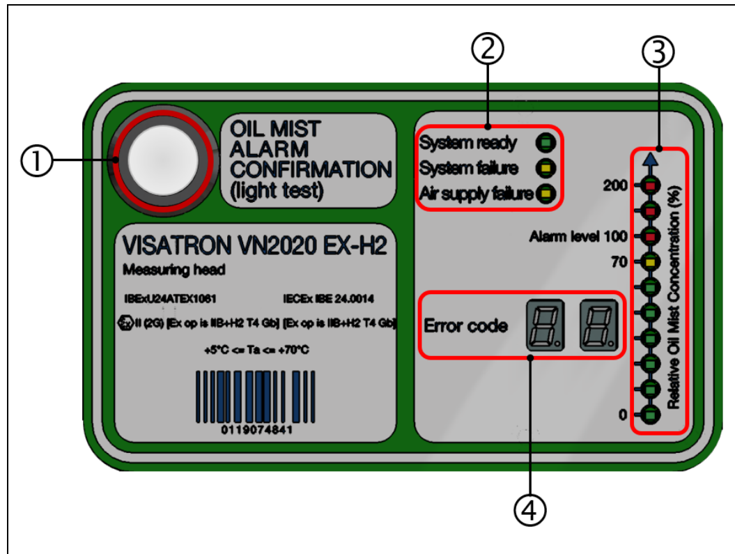
Fig.: 14 : Controls and indicators, VN2020 EX-H2
