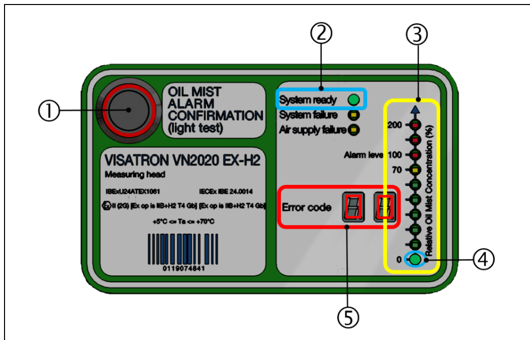
Fig.: 56 : VN2020 EX-H2 measuring head: Display in normal operation
