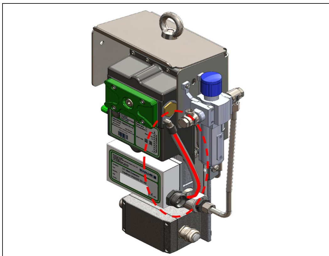
Fig.: 79 : Connecting hose, VN2020 EX-H2 oil mist detector
