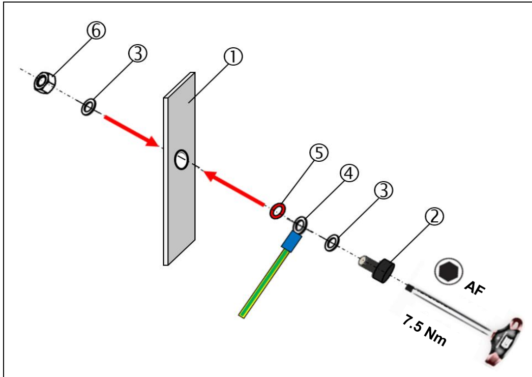
Fig.: 43 : Installing the earth connection, VN2020 series
