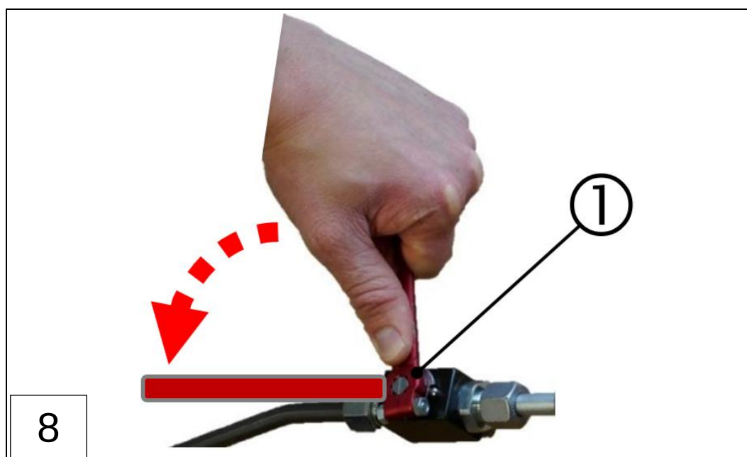
Fig.: 78 : Replacing the filter control valve (steps 1-8)
