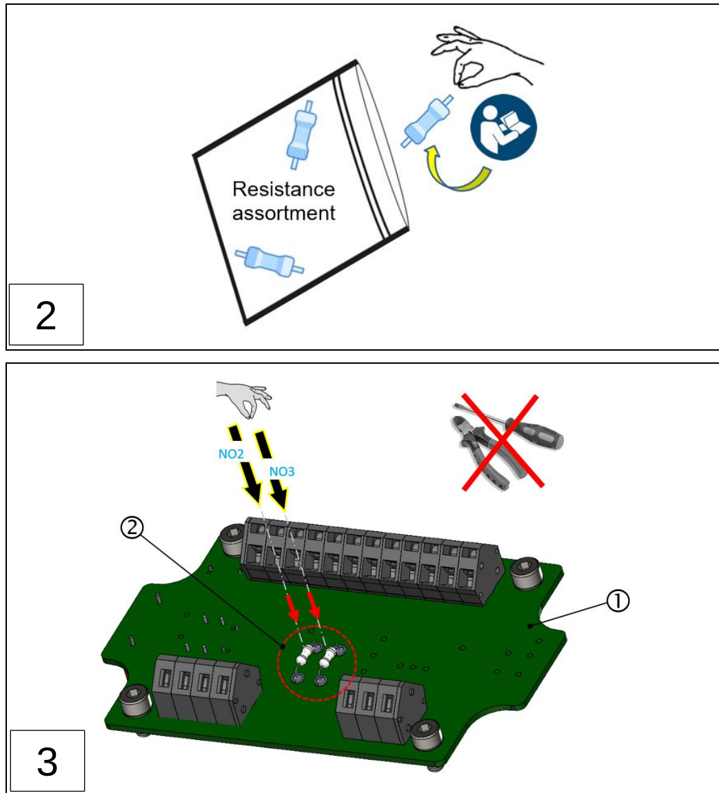
Fig.: 33 : VN2020 EX-H2 terminal box: Installing wire break resistors (steps 1-3)
