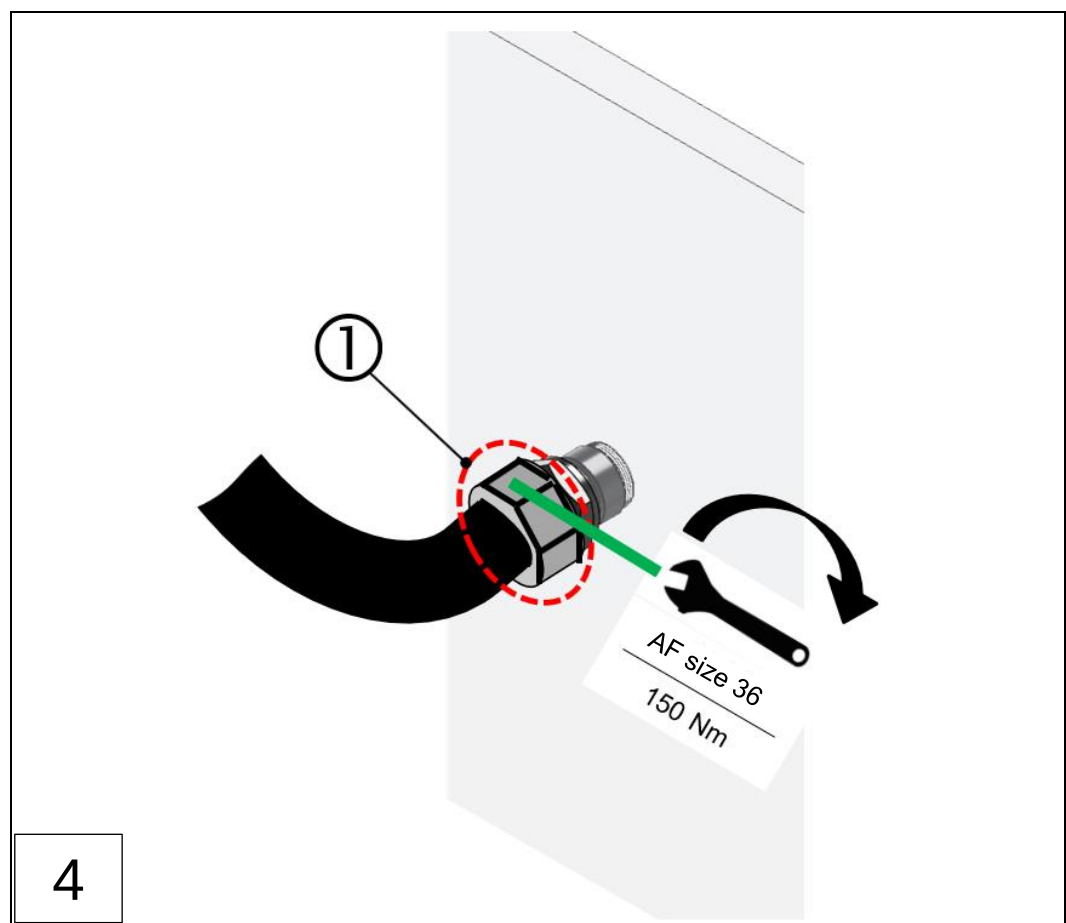
Fig.: 25 : Installing the recirculation line on the VN2020 EX-H2 (steps 1-4)
