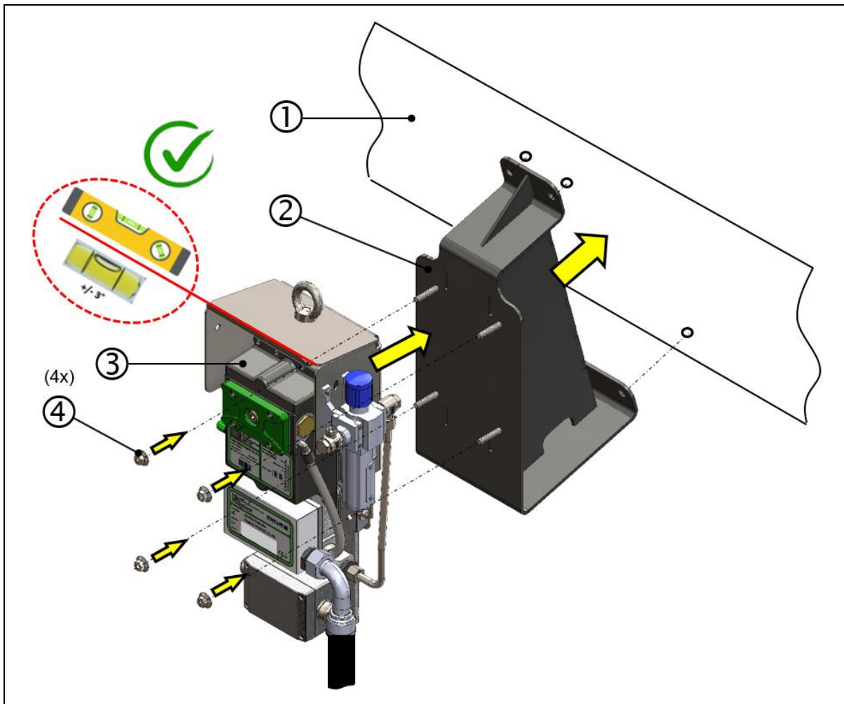
Fig.: 15 : Installing the VN2020 EX-H2 with bracket and protective cover
