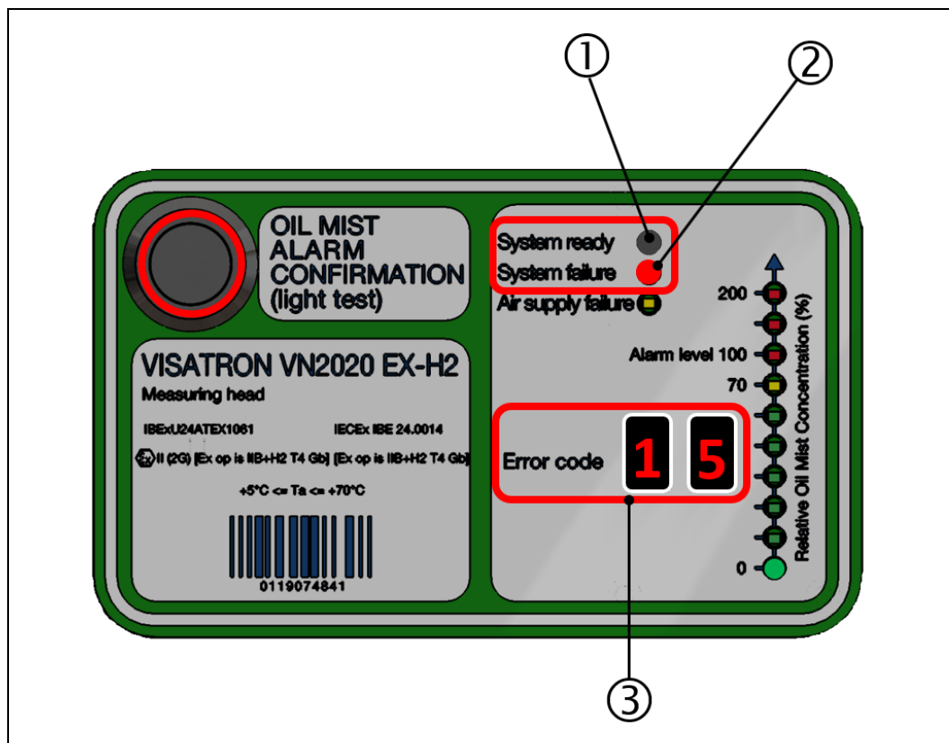
Fig.: 61 : “Sensor cleaning” status display, VN2020 EX-H2
