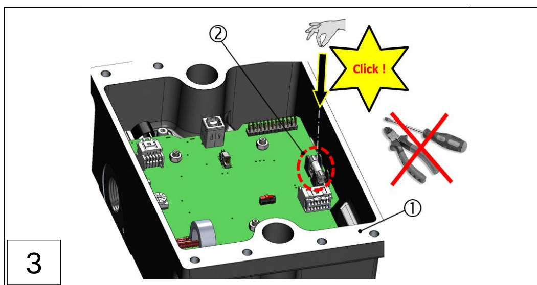
Fig.: 72 : Replacing the fuse on the VN2020 EX-H2 measuring head (steps 1-3)
