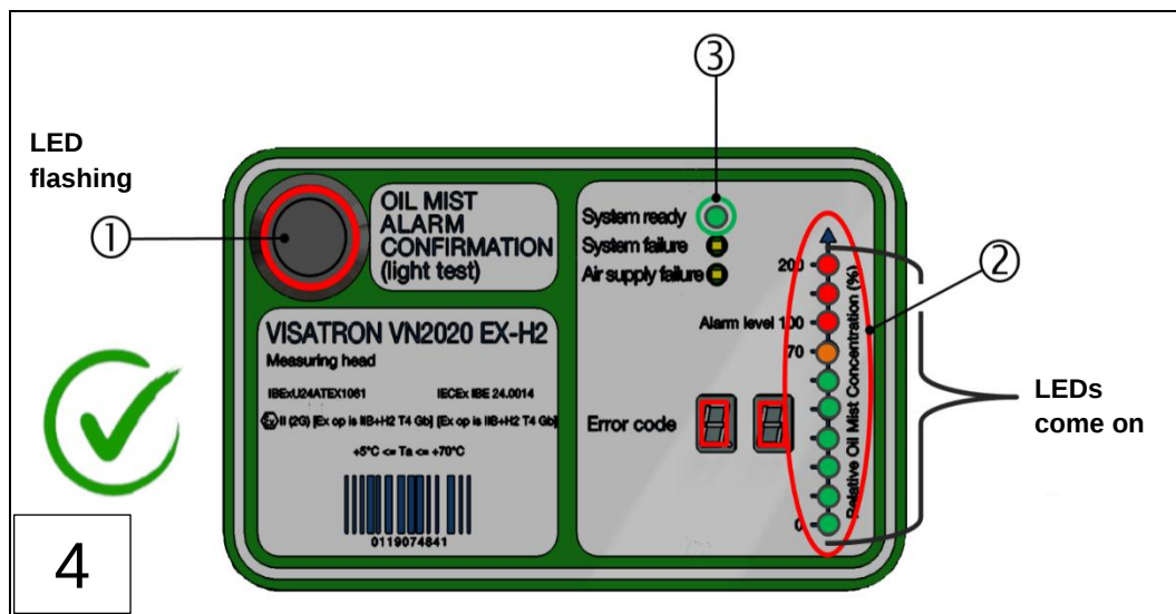
Fig.: 67 : Function test with test mist (steps 1-4)
