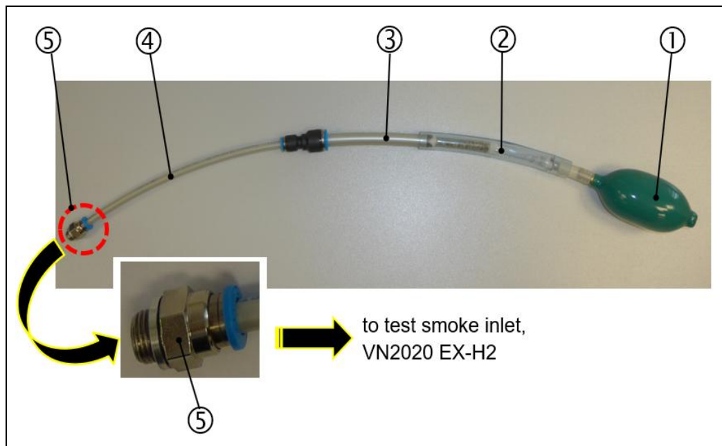
Fig.: 66 : Smoke tube with hand pump (assembled) from Smoke Test Box (151780)
