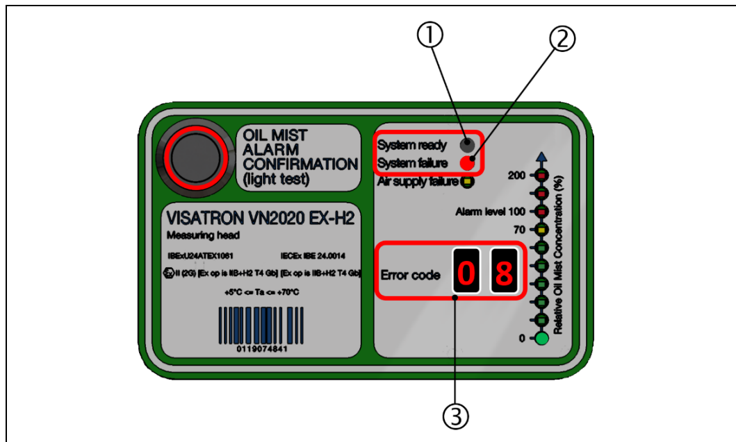
Fig.: 81 : VN2020 EX-H2 measuring head: "System or device error" status indicator
