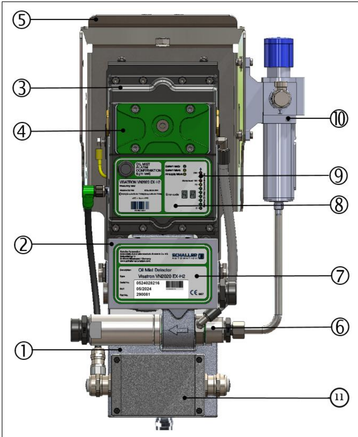
Fig.: 7 : Component overview for the VISATRON® VN2020 EX-H2 oil mist detector
