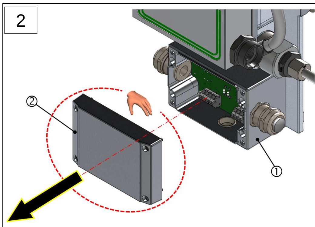
Fig.: 31 : VN2020 EX-H2 terminal box: Removing the cover (installation steps 1-2)
