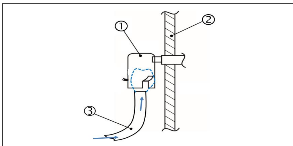
Fig.: 50 : Smoke generator, factory test, VN2020 EX-H2
