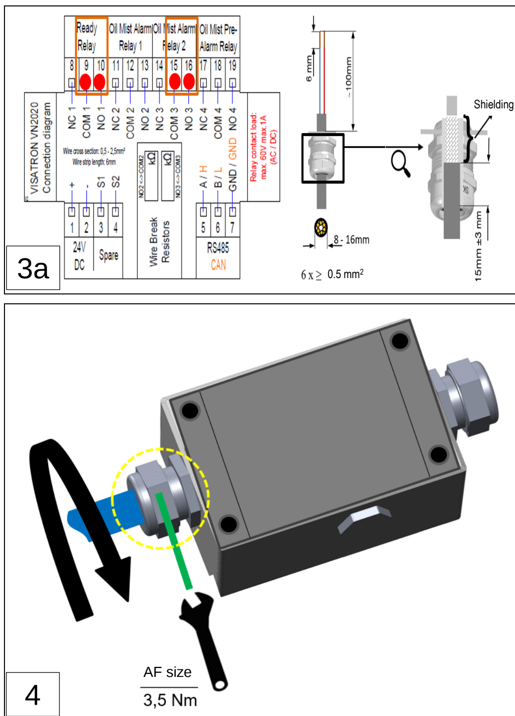
Fig.: 37 : Establishing the power and relay supply (example installation; installation steps 1-4)
