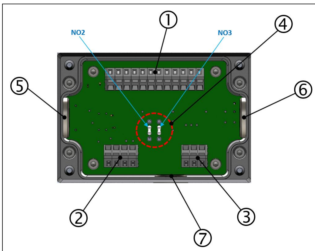
Fig.: 30 : Connection board, VN2020 EX-H2 terminal box
