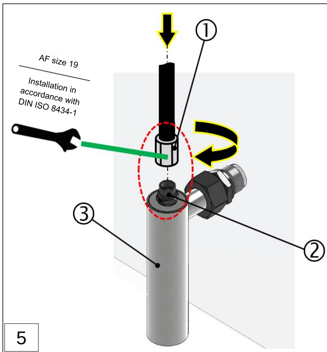
Fig.: 22 : Installing and starting up the pipe siphon assembly (installation steps 1-5)
