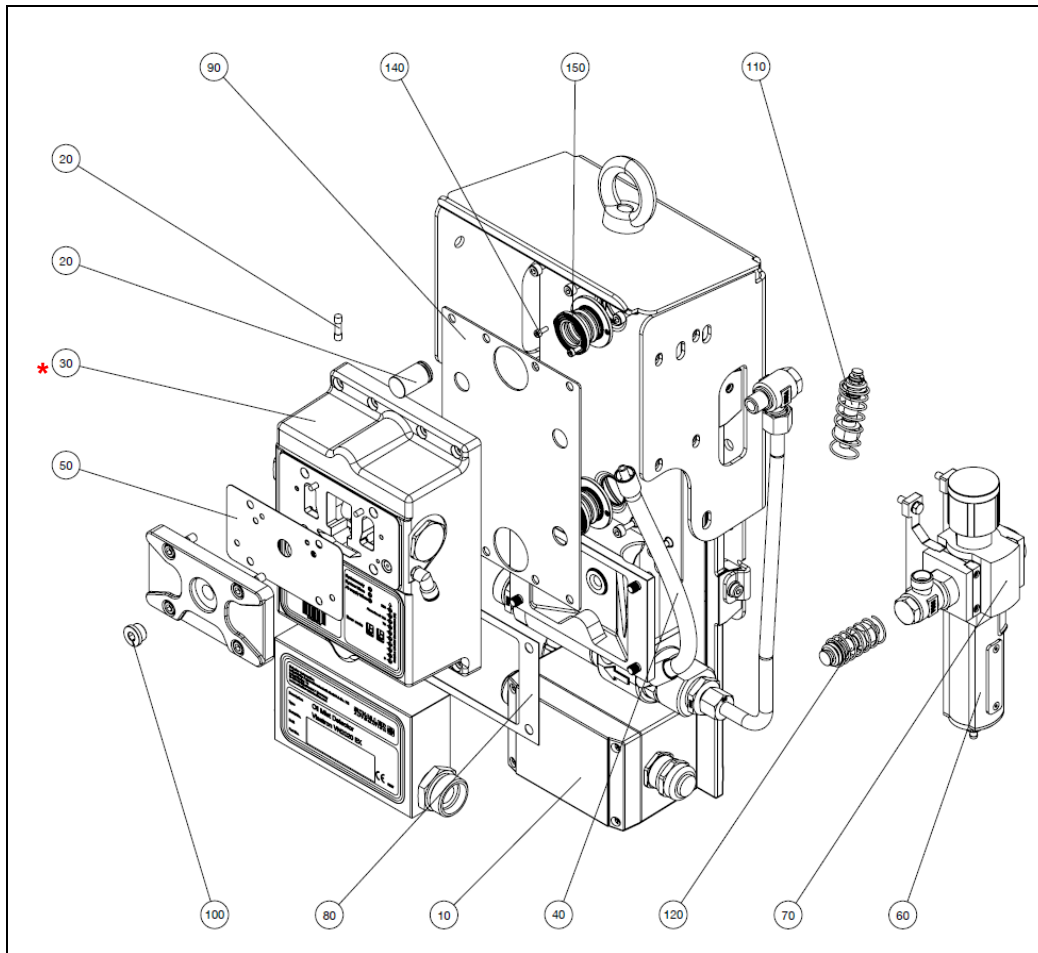
Fig.: 82 : Overview of the positions of spare parts for the VISATRON® VN2020 EX-H2
