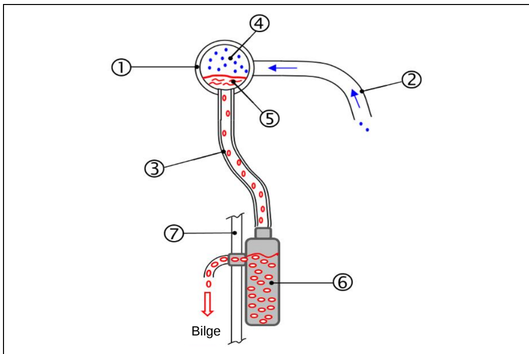
Fig.: 12 : Functional principle of oil drainage via pipe siphon, VN2020 series
