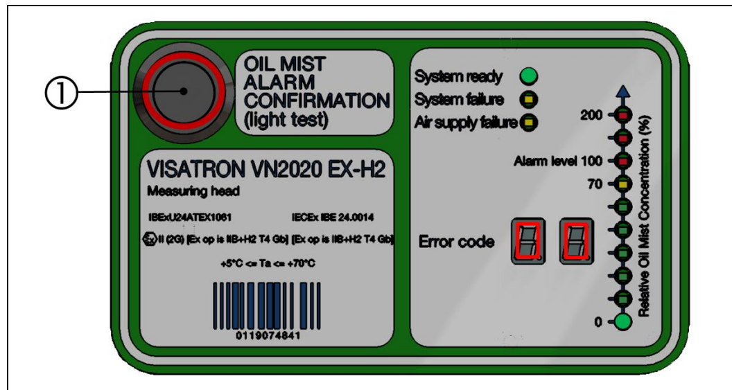
Fig.: 57 : VN2020 EX-H2 measuring head: LED check (light test)
