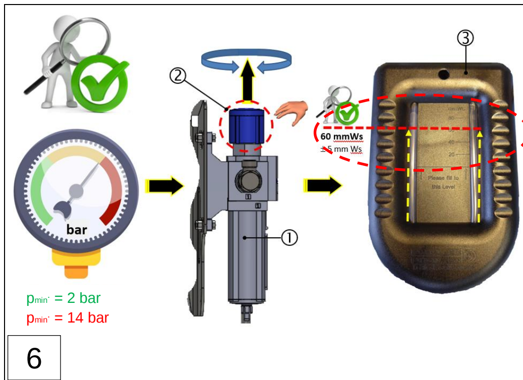
Fig.: 45 : Setting the negative pressure on the VN2020 EX-H2 measuring head (steps 1-6)
