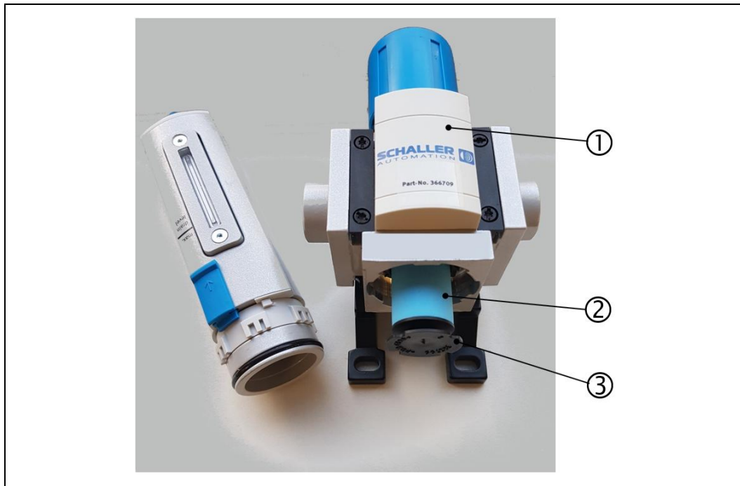
Fig.: 64 : Replacing the air filter element on the pressure regulator unit
