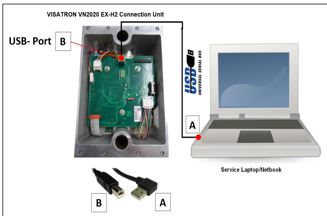
Fig.: 54 : Establishing, USB connection between the VN2020 EX-H2 measuring head and PC
