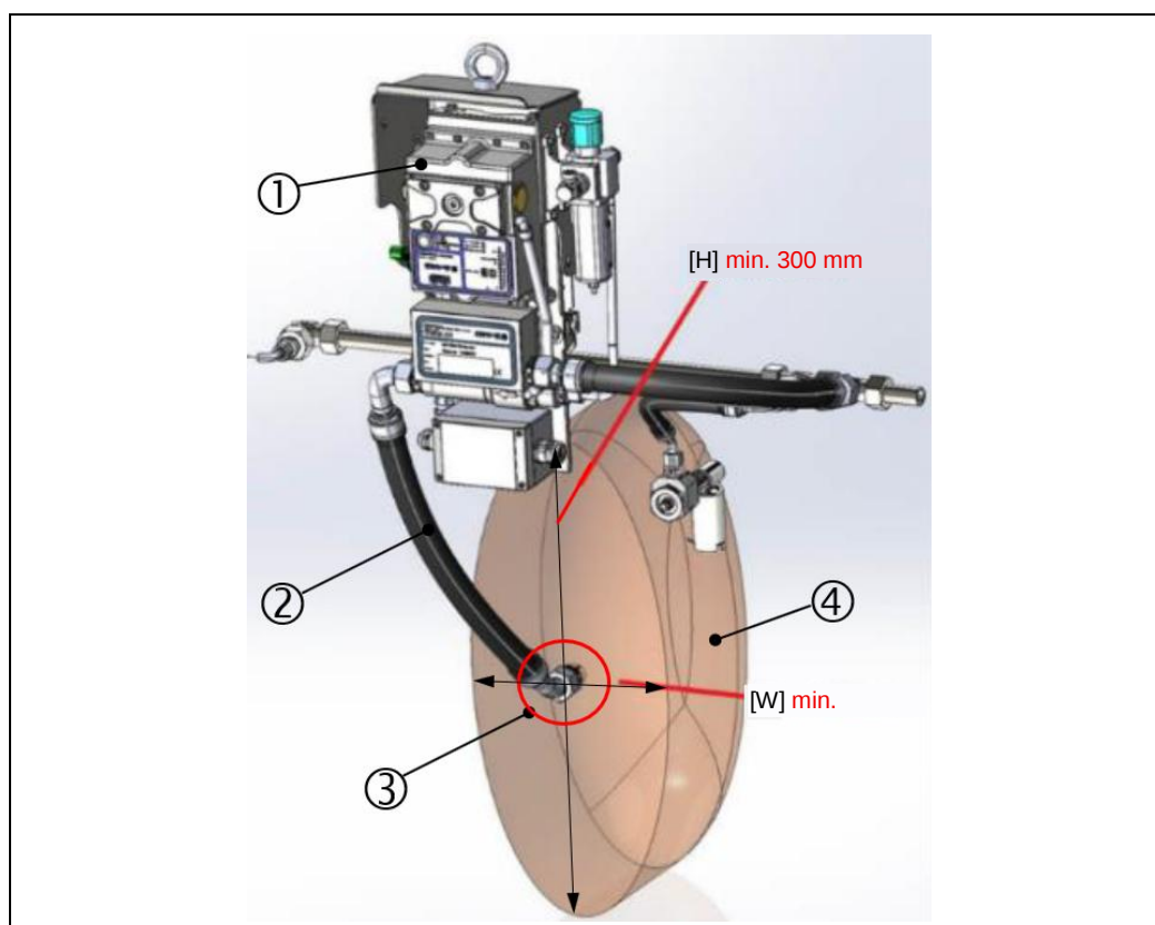
Fig.: 24 : Position of the recirculation pipe on the VN2020 EX-H2
