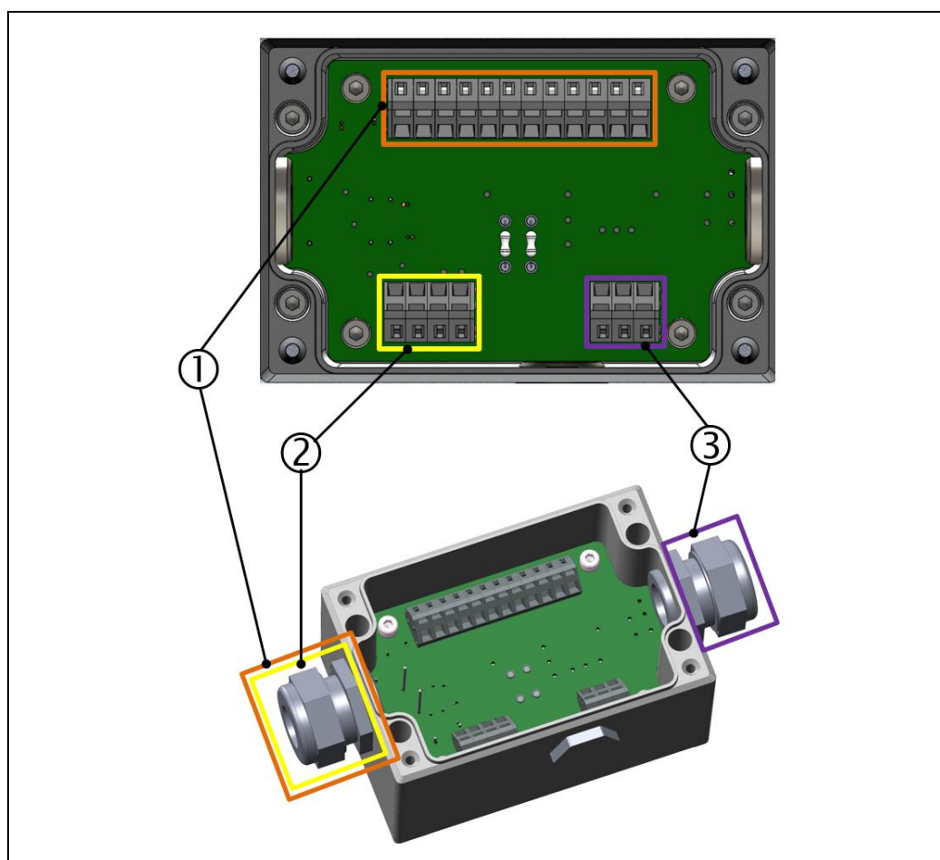
Fig.: 35 : Electrical connection of terminal box (example installation), VN2020 EX-H2
