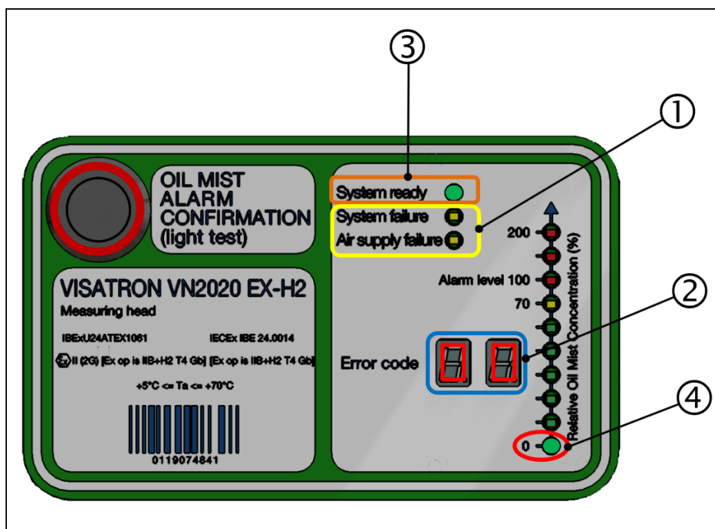
Fig.: 44 : “System ready” indicator on the VN2020 EX-H2 measuring head
