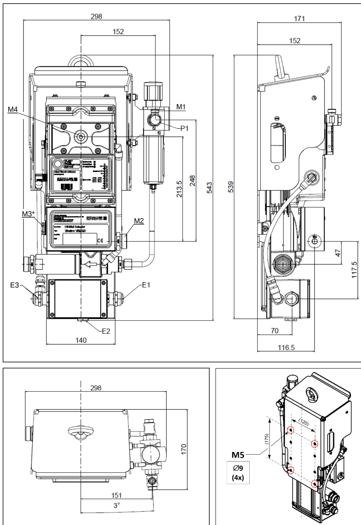
Fig.: 5: Mechanical dimensions, VISATRON® VN2020 EX-H2
