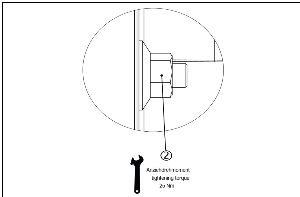
Fig.: 17 : ROMOB M8, installed
