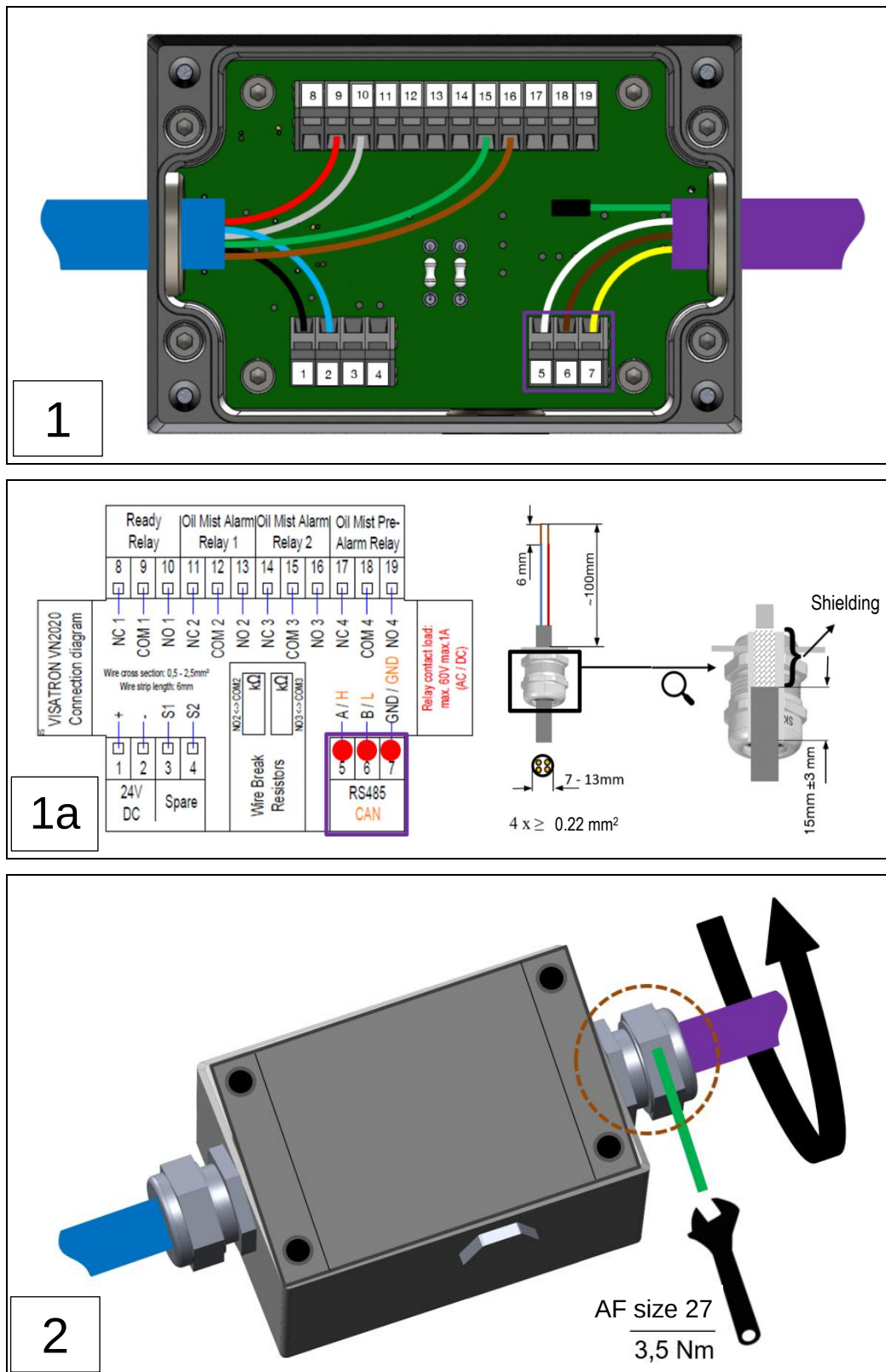
Fig.: 38 : Connecting the Remote Indicator II to terminal box (example inst.; install. steps 1-2)
