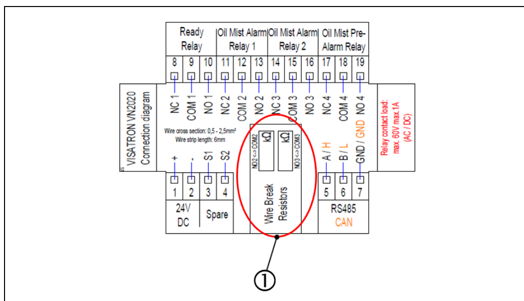
Fig.: 32 : VN2020 EX-H2 terminal box: Configuration of the wire break resistors
