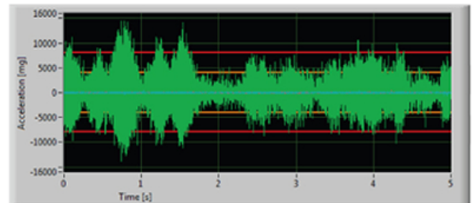
Live signal of the sensor, in this case in mg over time
