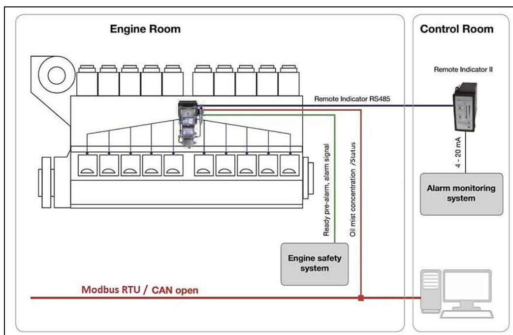
Fig.: 41 : Connection diagram for VN2020
