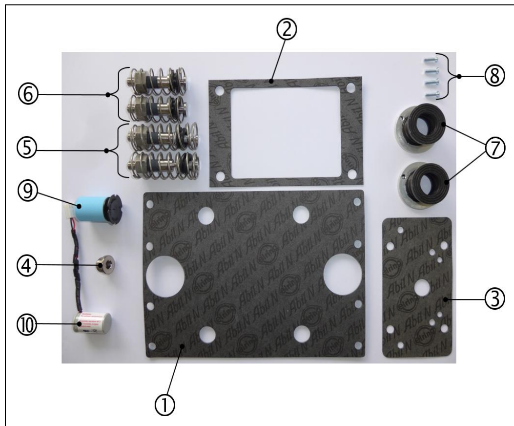
Fig.: 99 : Service kit for the VISATRON® VN2020/VN2020 EX
