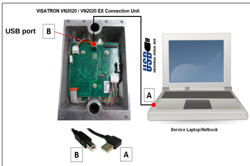
Fig.: 67 : Establishing the USB connection between the VN2020 measuring head and PC
