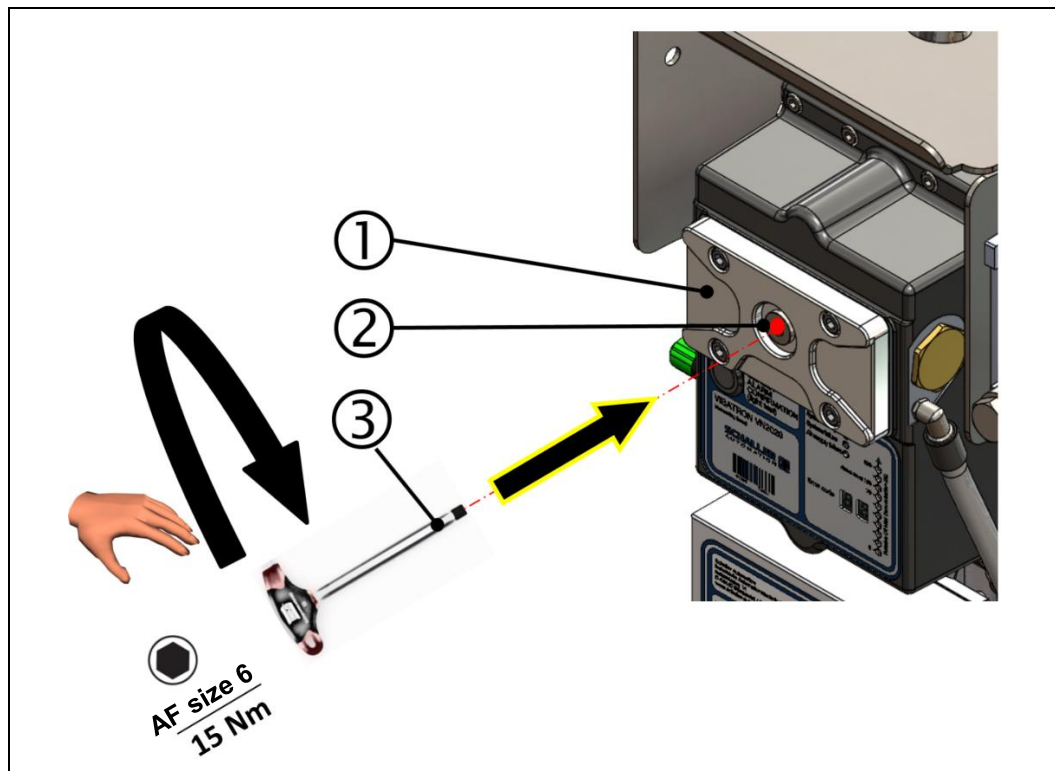
Fig.: 58 : Screwing in the screw plug on the measuring head of the VN2020/VN2020 EX
