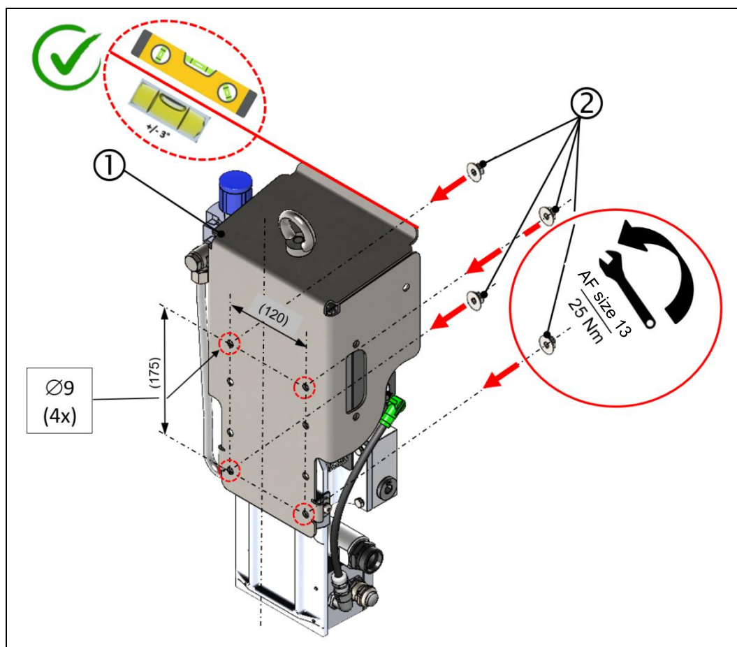
Fig.: 25 : Installing VN2020 without bracket and with protective cover (rear view)
