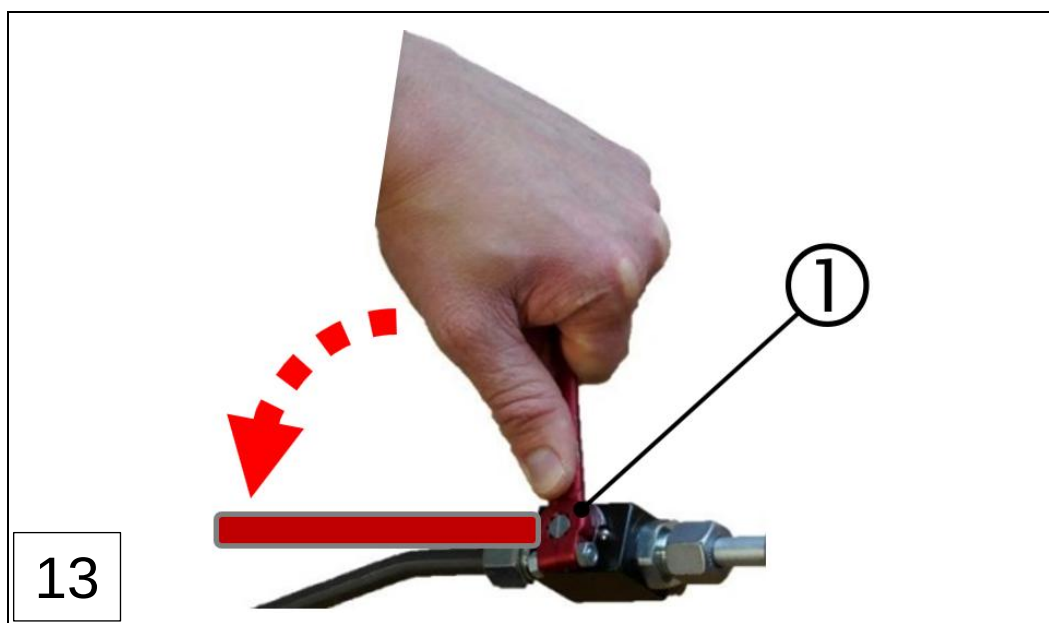
Fig.: 82 : Replacing the seal on the connecting box (steps 1- 13), VN2020
