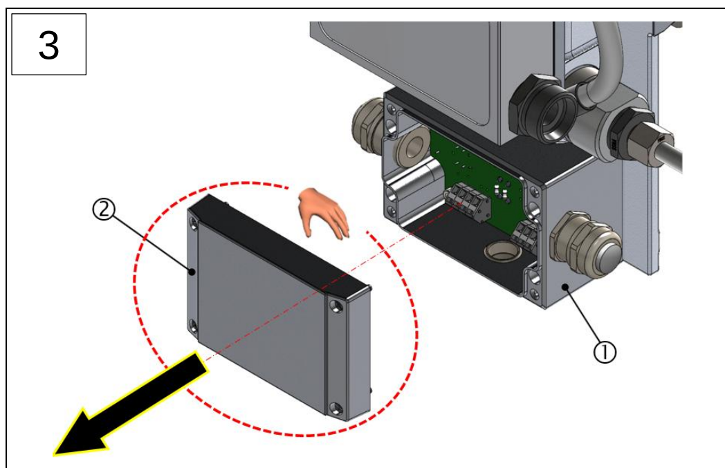
1: VN2020 terminal box
