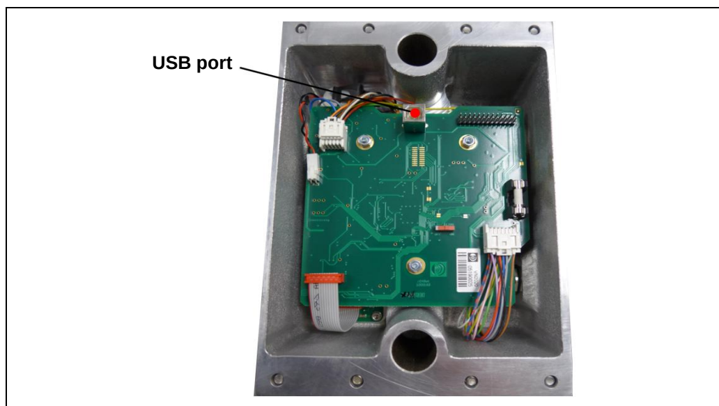
Fig.: 65 : Measuring head for VN2020, rear view, USB port
