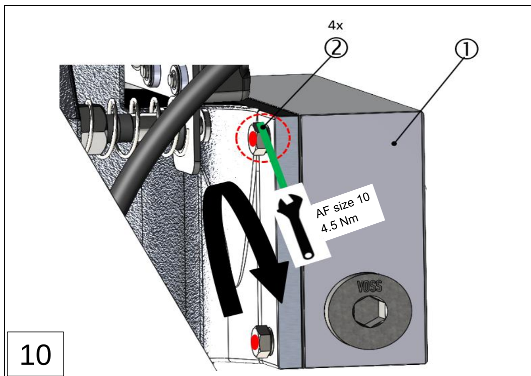
1: Connecting box
