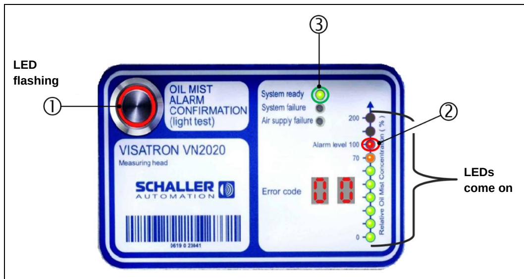
Fig.: 72 : VN2020 measuring head: “Alarm” status indicator at 100% OMC
