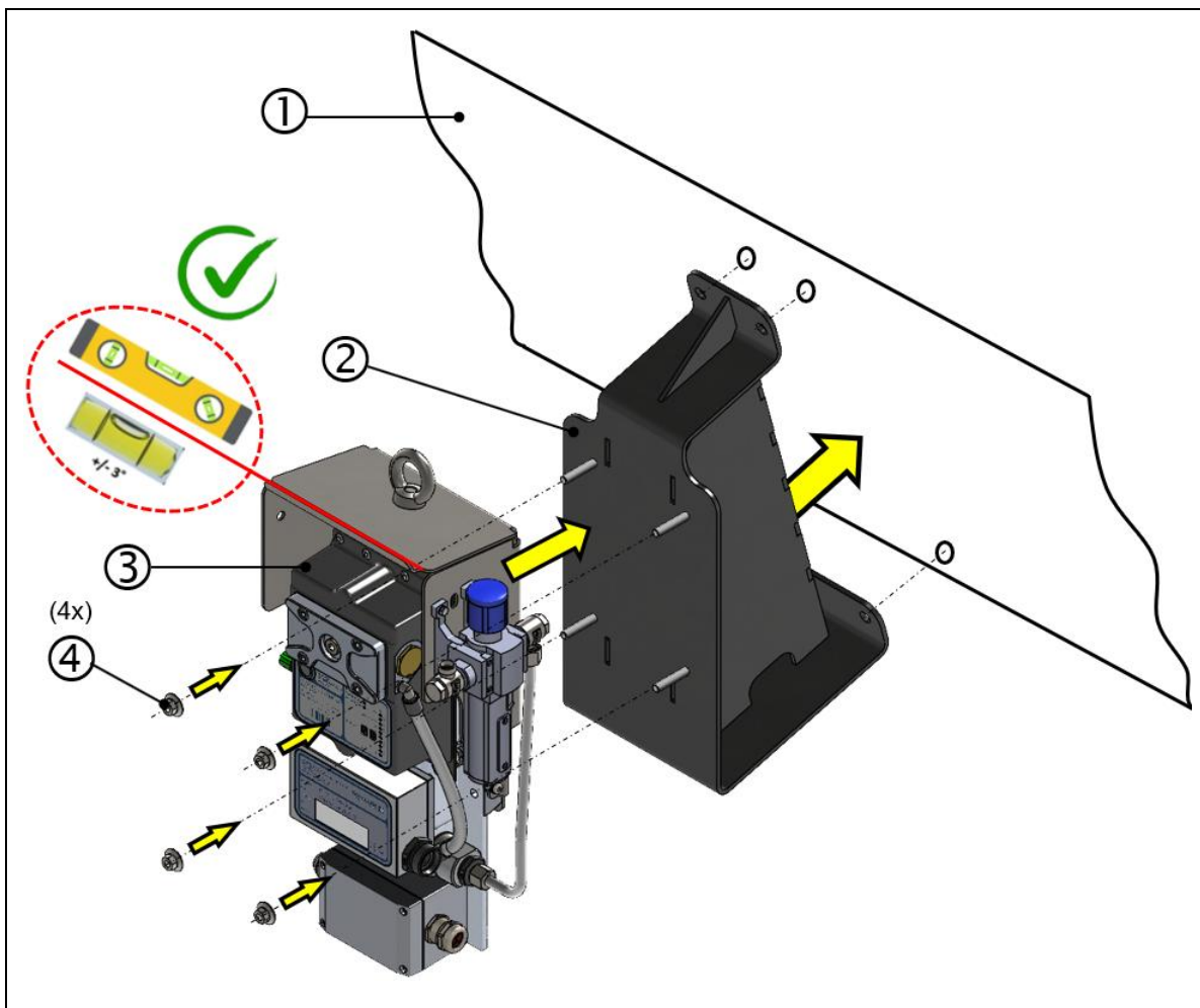
Fig.: 24 : Installing VN2020 with bracket and protective cover
