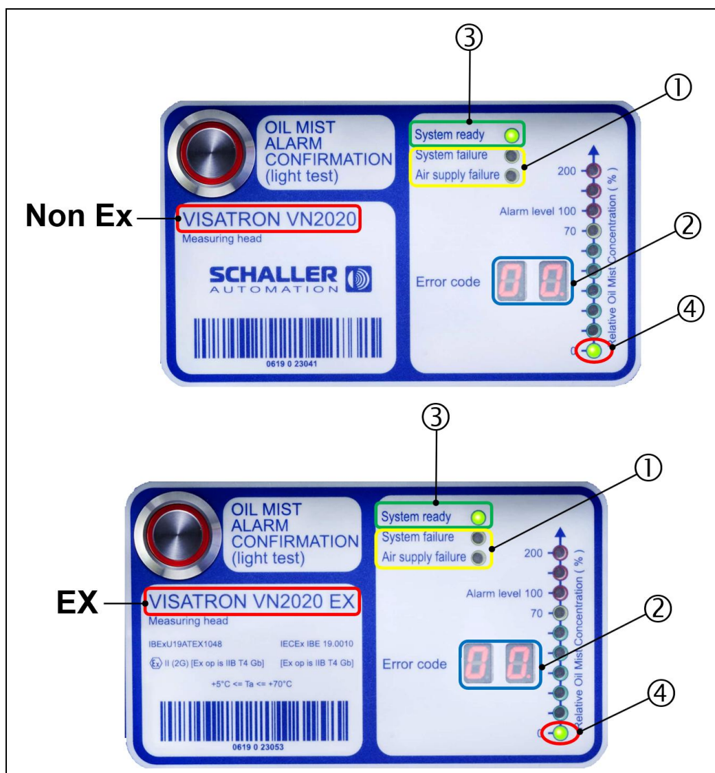
Fig.: 56 : “System ready” indicator on the VN2020/VN2020 EX measuring head
