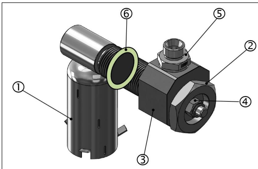
Fig.: 27 : Engine wall connection (EWC)
