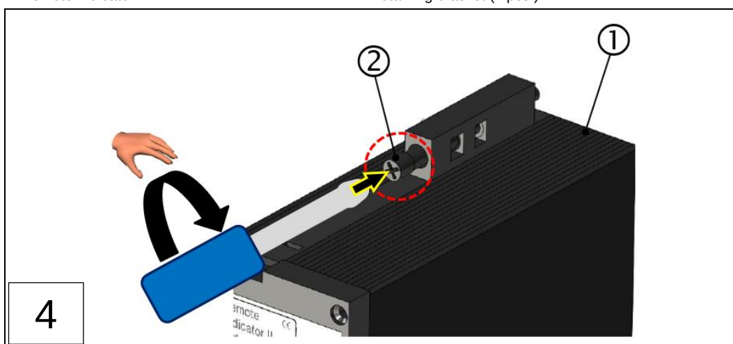
Fig.: 40 : Installing Remote Indicator II (installation steps 1-4)
