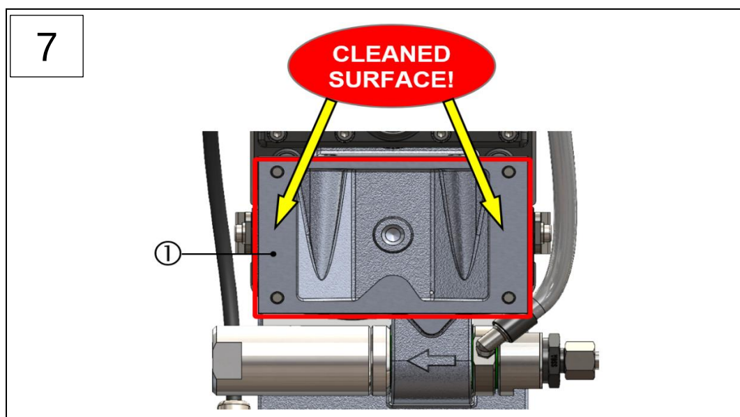
1: Connecting box sealing surface
