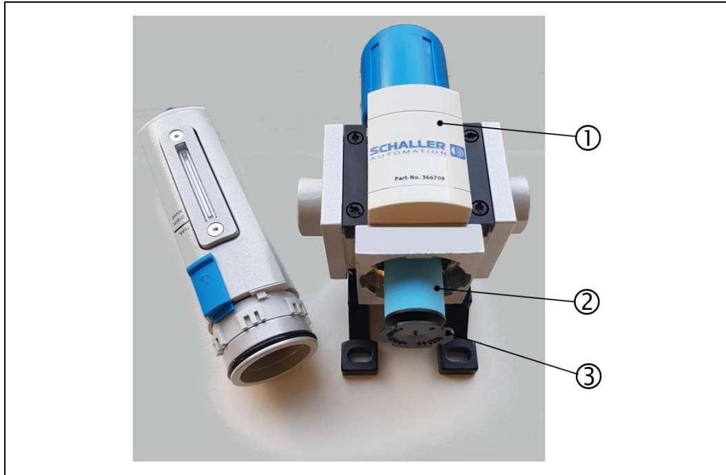
Fig.: 77 : Replacing the air filter element on the pressure regulator unit
