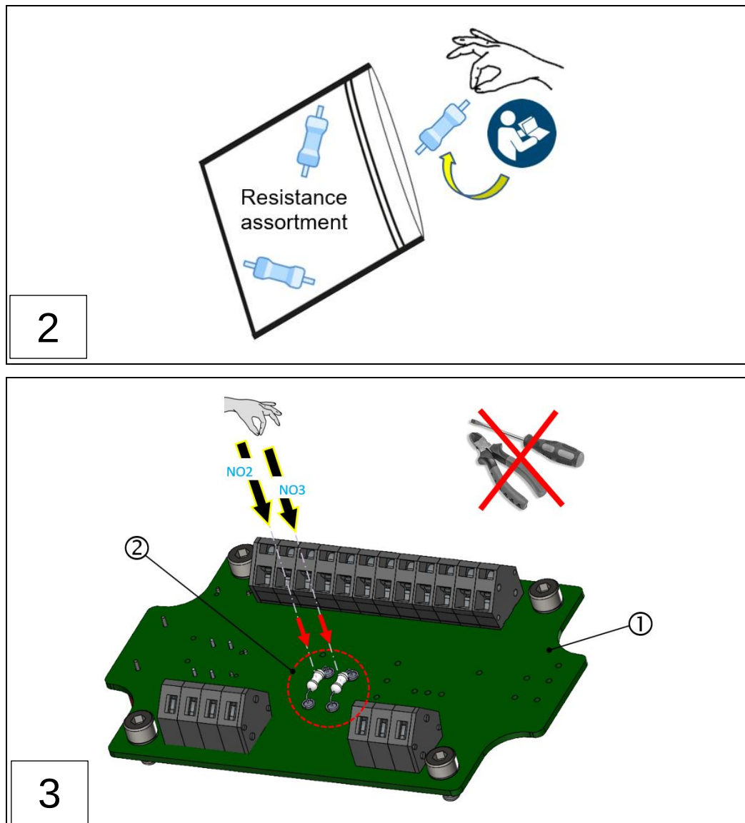
Fig.: 45 : VN2020 terminal box: Inserting the wire break resistors (installation steps 1-3)
