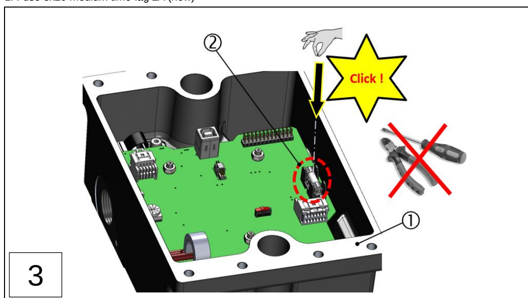
Fig.: 85 : Replacing the fuse on the VN2020 measuring head (steps 1-3)
