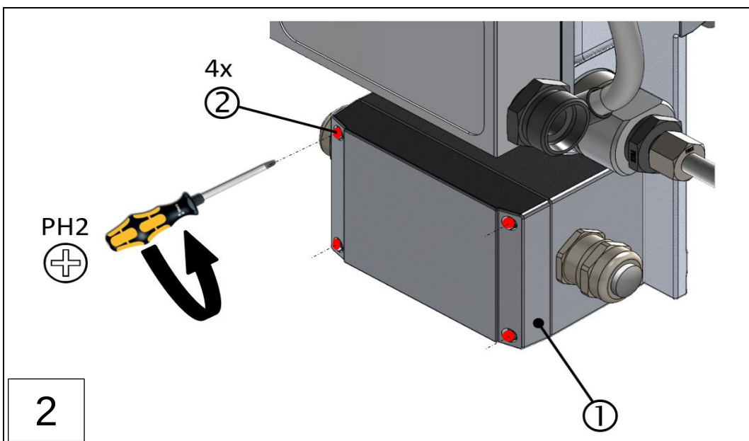
1: Cover, VN2020 terminal box
