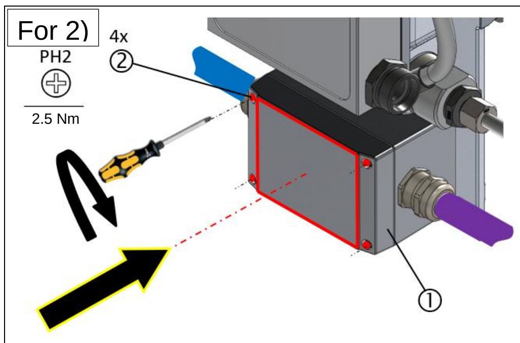
Fig.: 89 : Replacing the VN2020 terminal box (installation steps 1-8)
