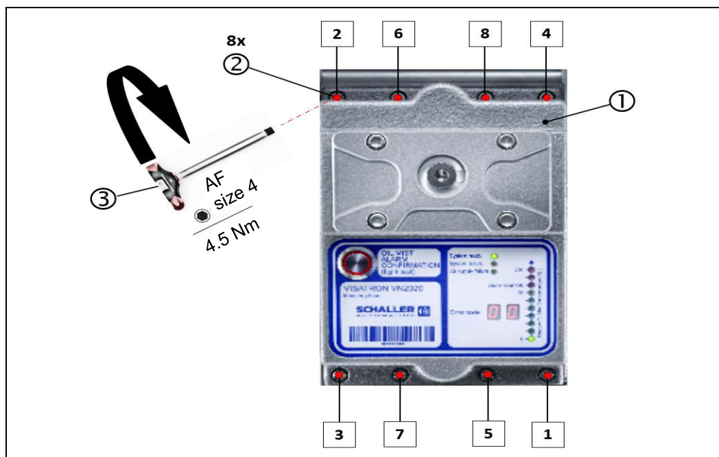
Fig.: 68 : Installing the VN2020 measuring head
