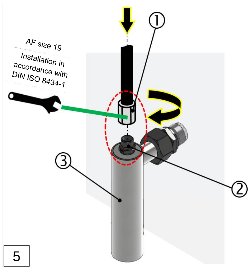
Fig.: 33 : Installing and starting up the pipe siphon assembly (installation steps 1-5)
