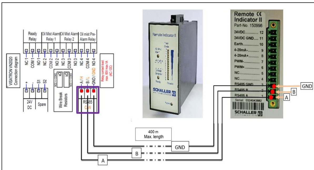
Fig.: 52 : Remote Indicator II (optional); installing contacts
