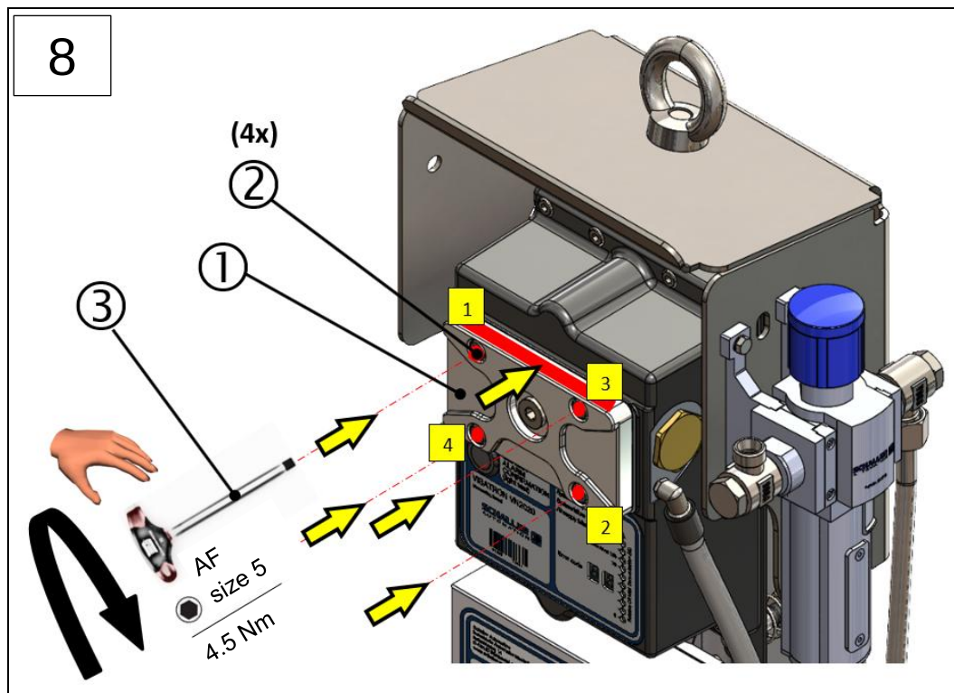
Fig.: 75 : Cleaning the light path of the VN2020 (steps 1-8)
