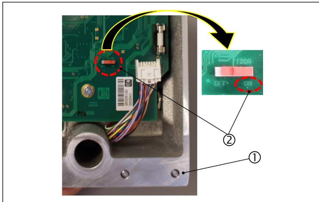
Fig.: 51 : Connection board for VN2020 measuring head
