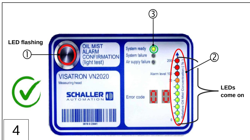
Fig.: 80 : Function test with test mist (steps 1-4)
