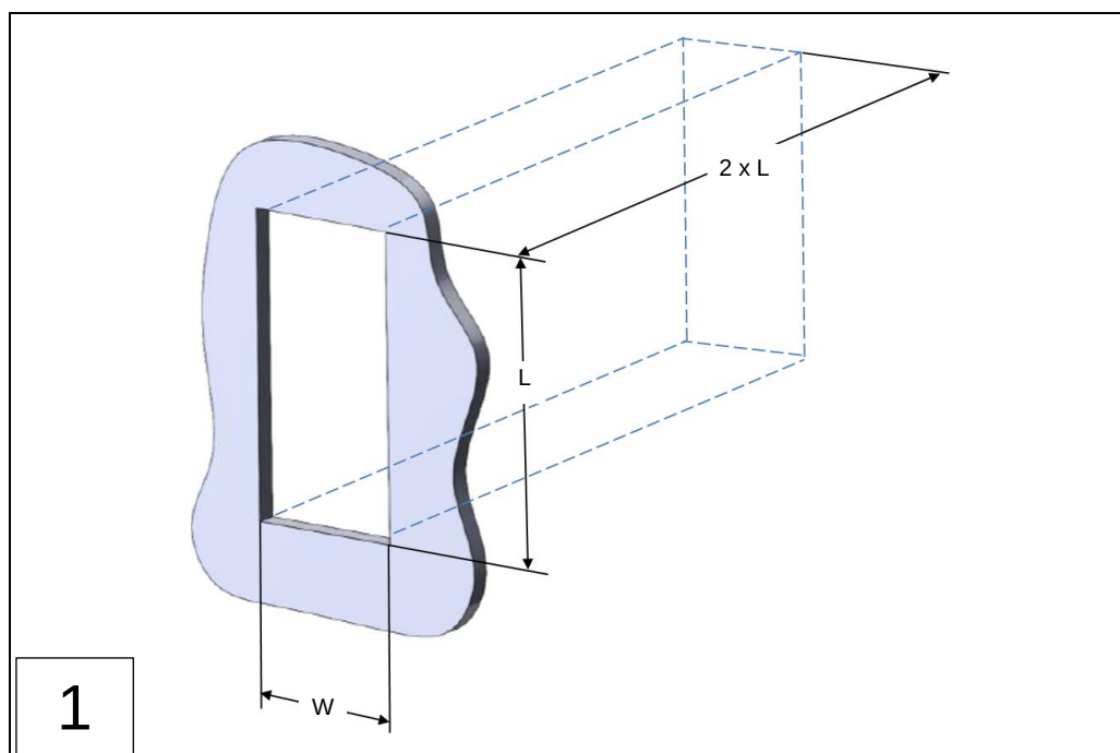
Fig.: 39 : Dimensions of installation space for Remote Indicator II
