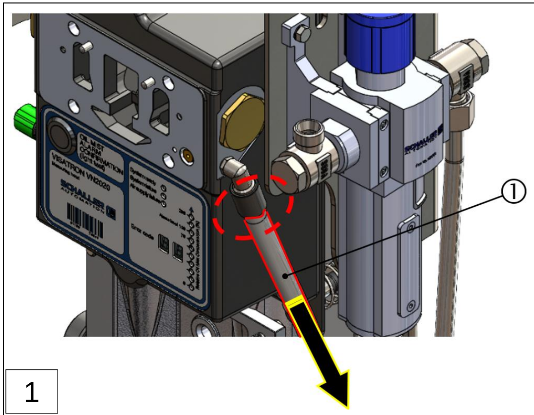
1: Installing the measuring head compressed air hose
