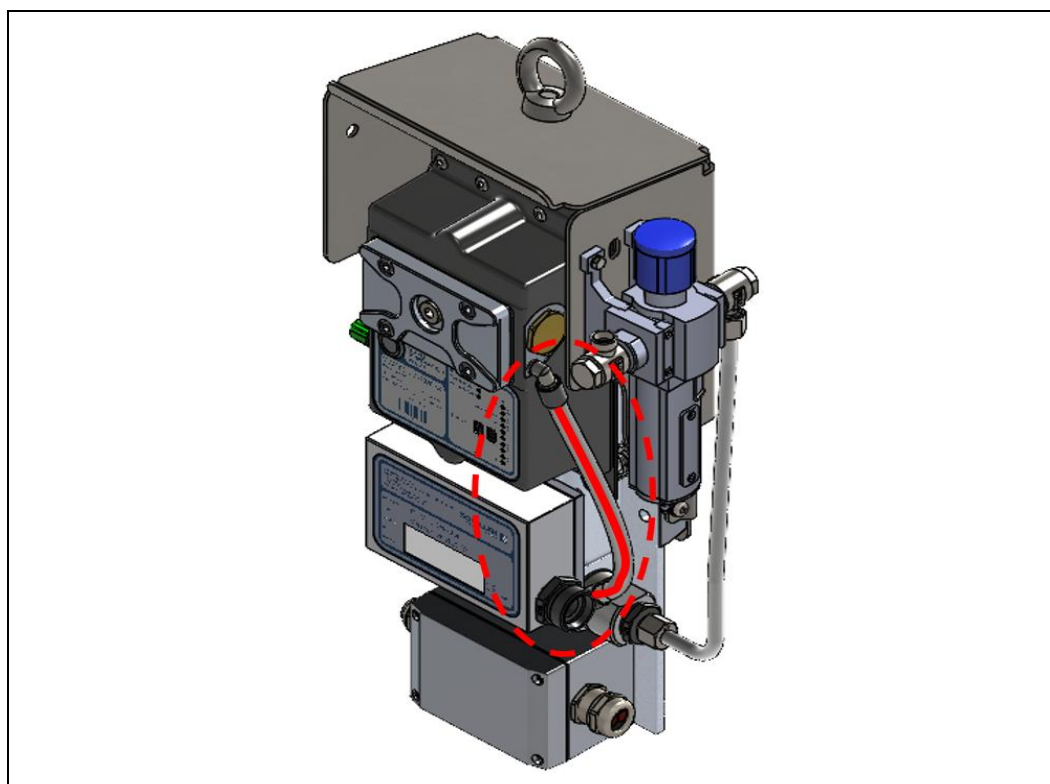
Fig.: 92 : Connecting hose, VN2020 oil mist detector
