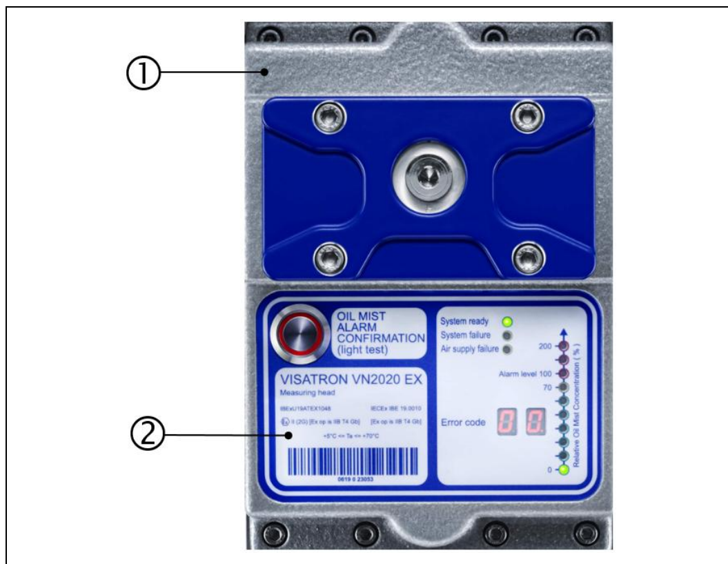
Fig.: 3 : Name plate, VISATRON® VN2020 EX measuring head
