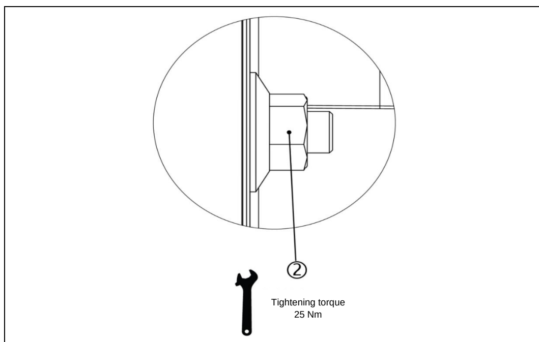
Fig.: 26 : ROMOB M8, installed
