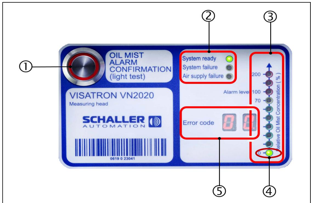
Fig.: 69 : VN2020 measuring head: Display in normal operation
