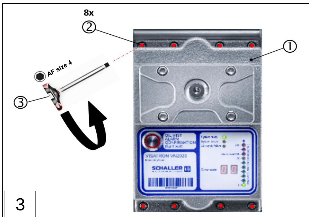
1: (Old) VN2020 measuring head 3: Allen key, size 4
