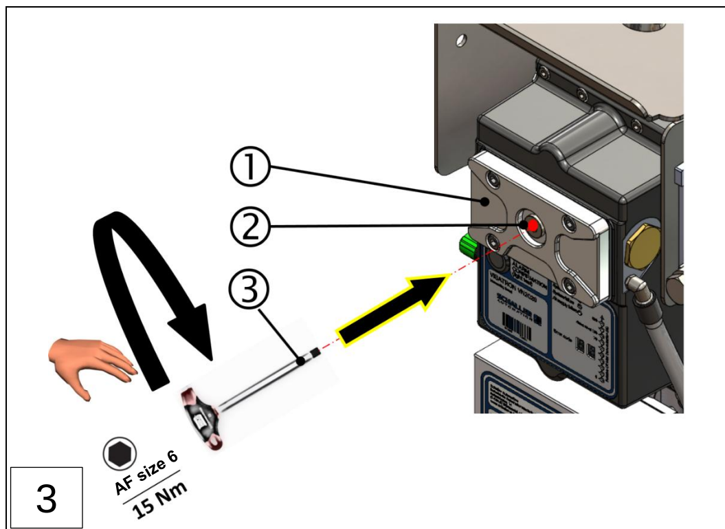
Fig.: 87 : Replacing the screw plug on the VN2020 measuring head (steps 1-3)
