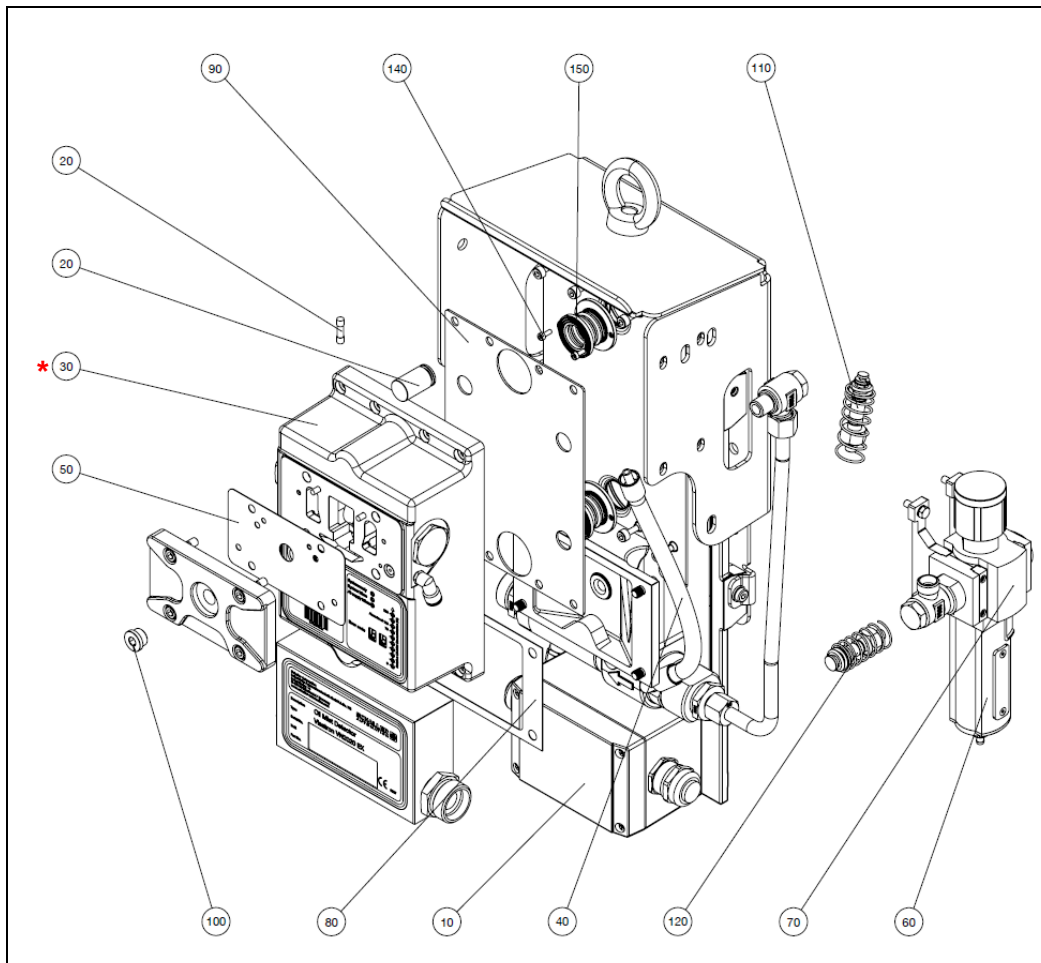
Fig.: 97 : Overview, positions of spare parts (kept in stock) for the VISATRON® VN2020 EX
