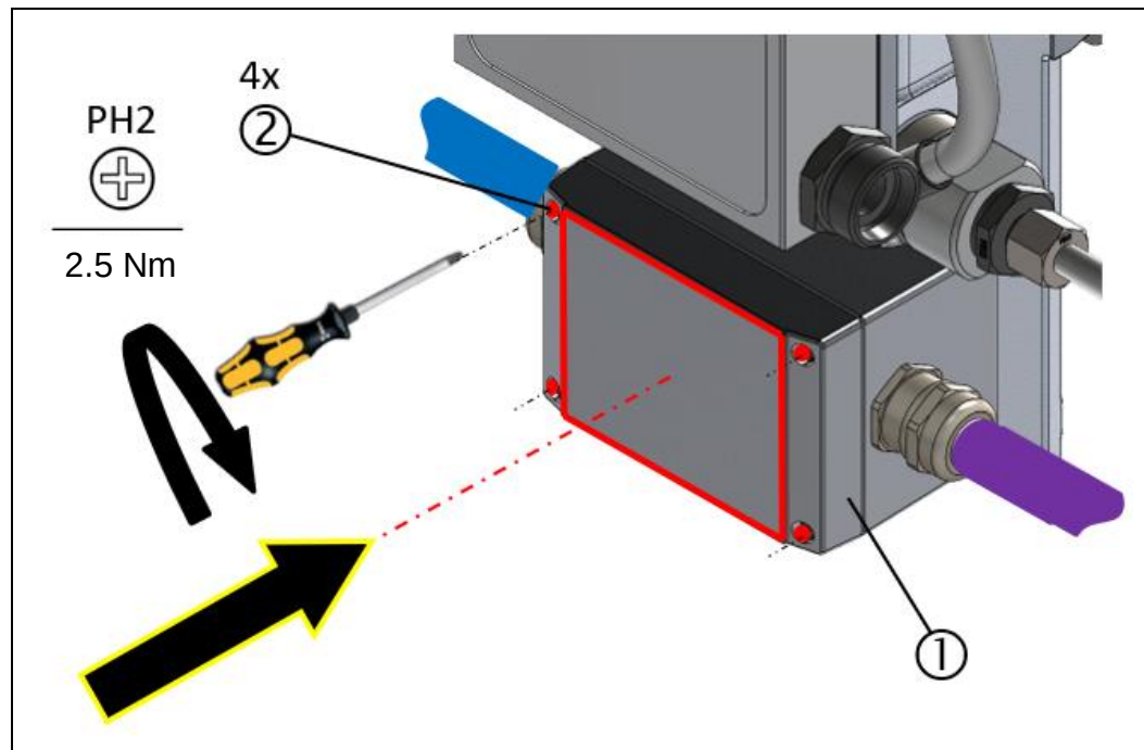
Fig.: 53 : Closing the terminal box for VN2020
