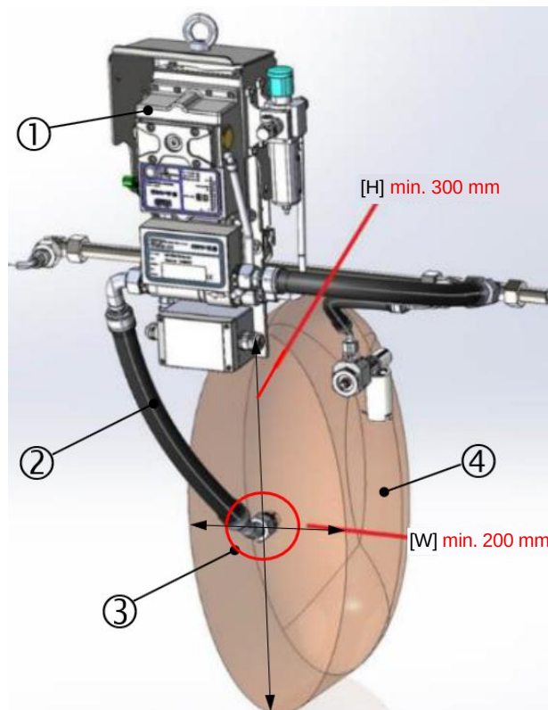
Fig.: 35 : Position of the recirculation line on the VN2020
