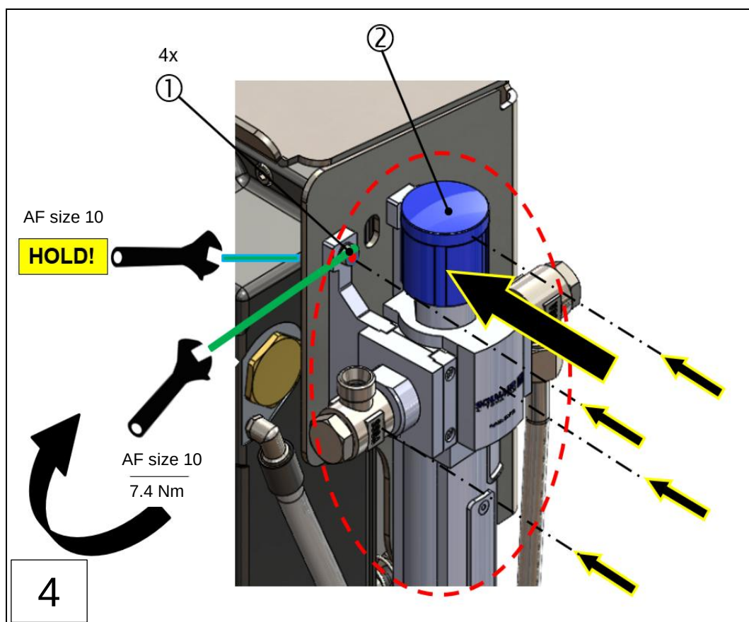
1: 4x fixing screws, full set (new)
