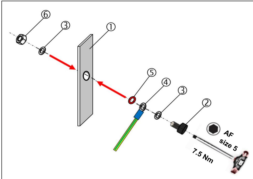
Fig.: 55 : Installing the earth connection, VN2020
