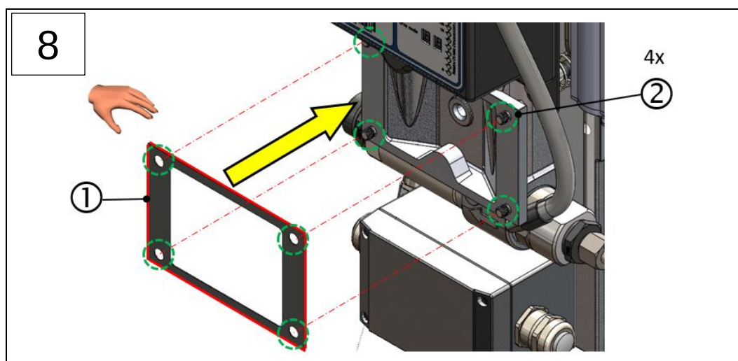
1: (New) connecting box seal
