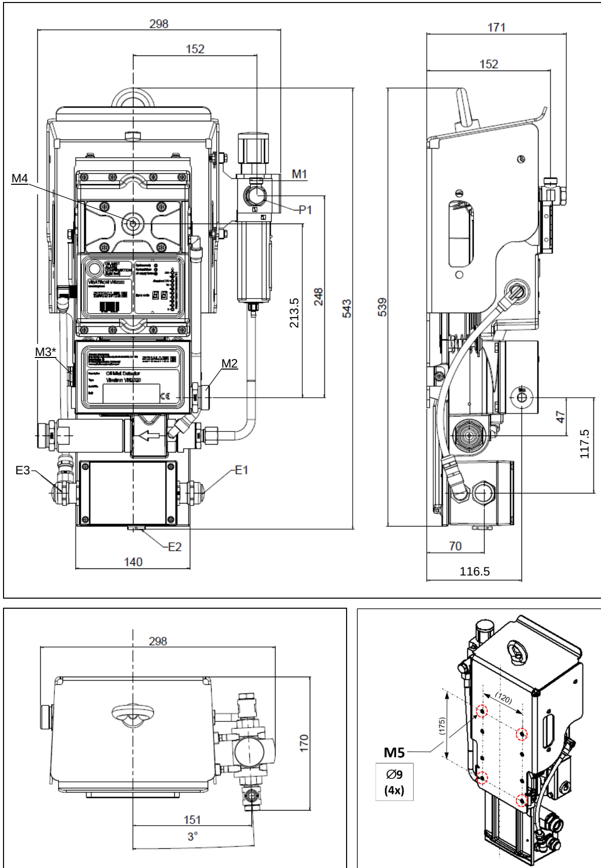
Fig.: 9: Mechanical dimensions, VISATRON® VN2020/VN2020 EX
