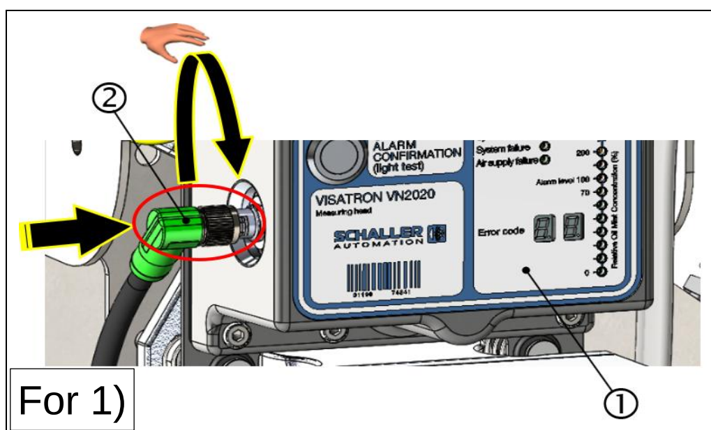
Fig.: 89 : Replacing the VN2020 terminal box (installation steps 1-8)
