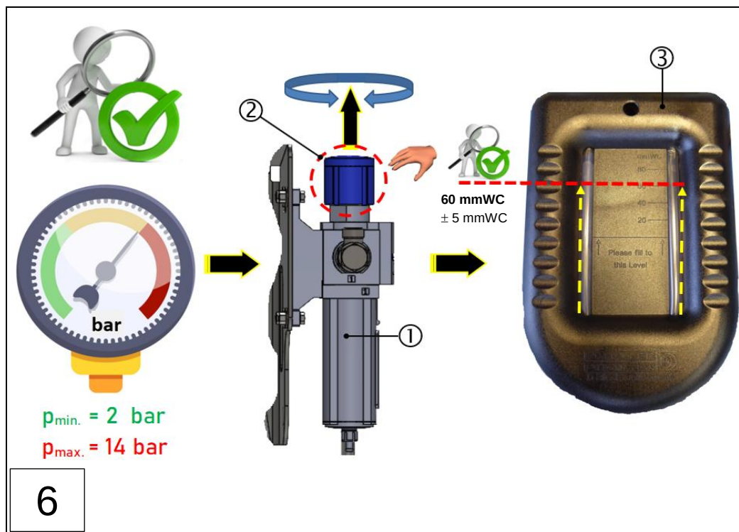
Fig.: 57 : Setting the negative pressure on the VN2020/VN2020 EX measuring head (steps 1-6)
