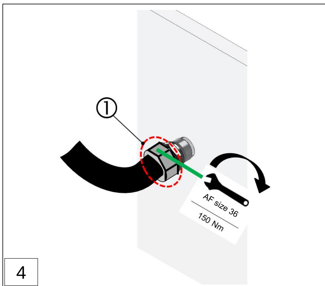
Fig.: 36 : Installing the recirculation line on the VN2020 (steps 1-4)
