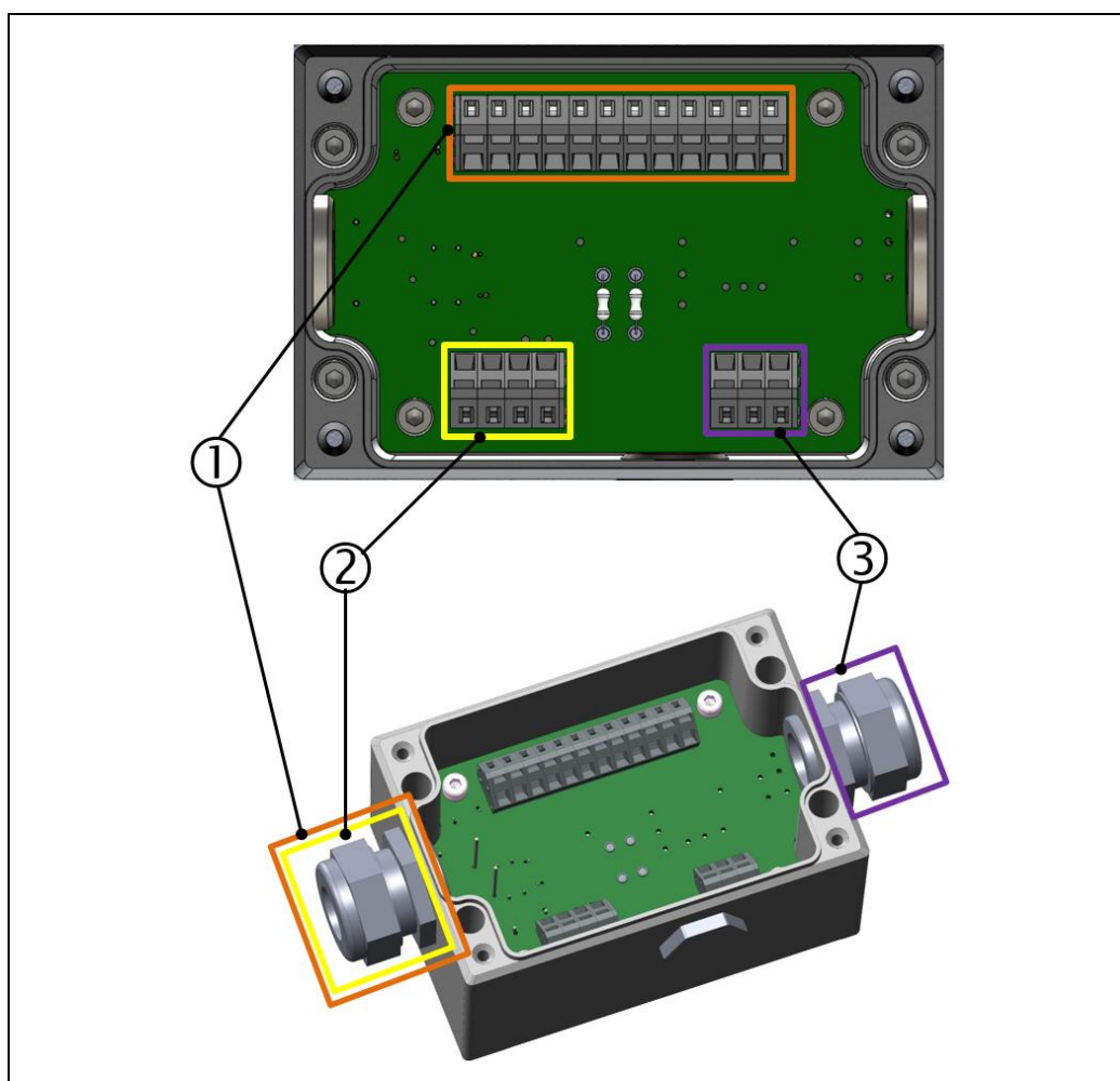
Fig.: 47 : Electrical connection terminal box (example installation), VN2020
