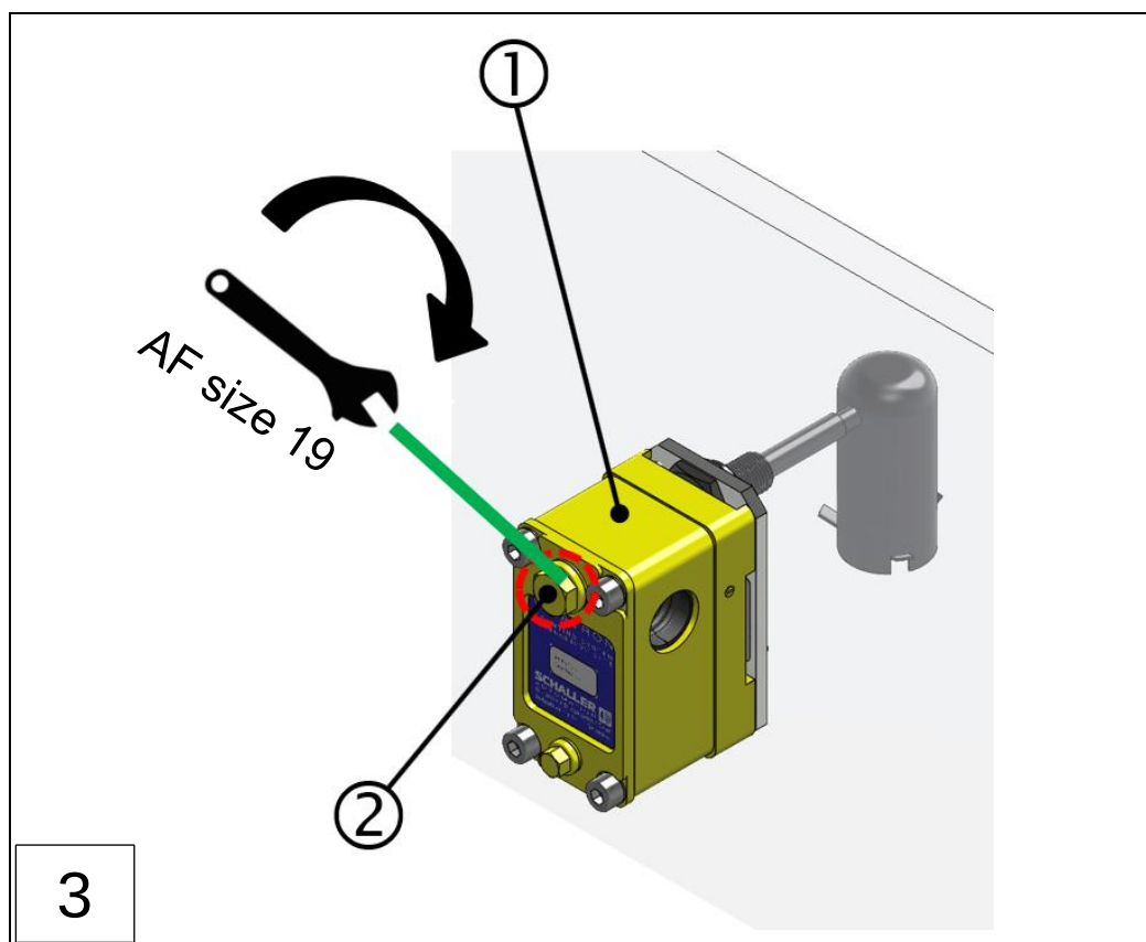
Fig.: 64 : Factory test with smoke generator (steps 1-3)
