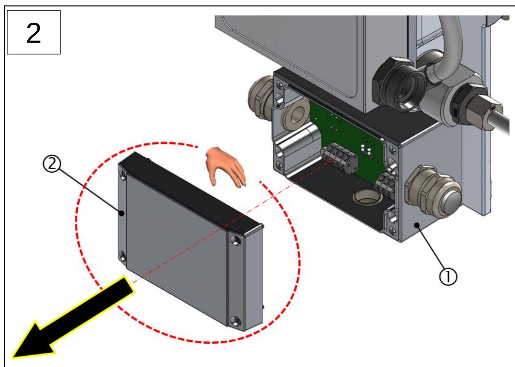
Fig.: 43 : VN2020 terminal box: Removing the cover (installation steps 1-2)
