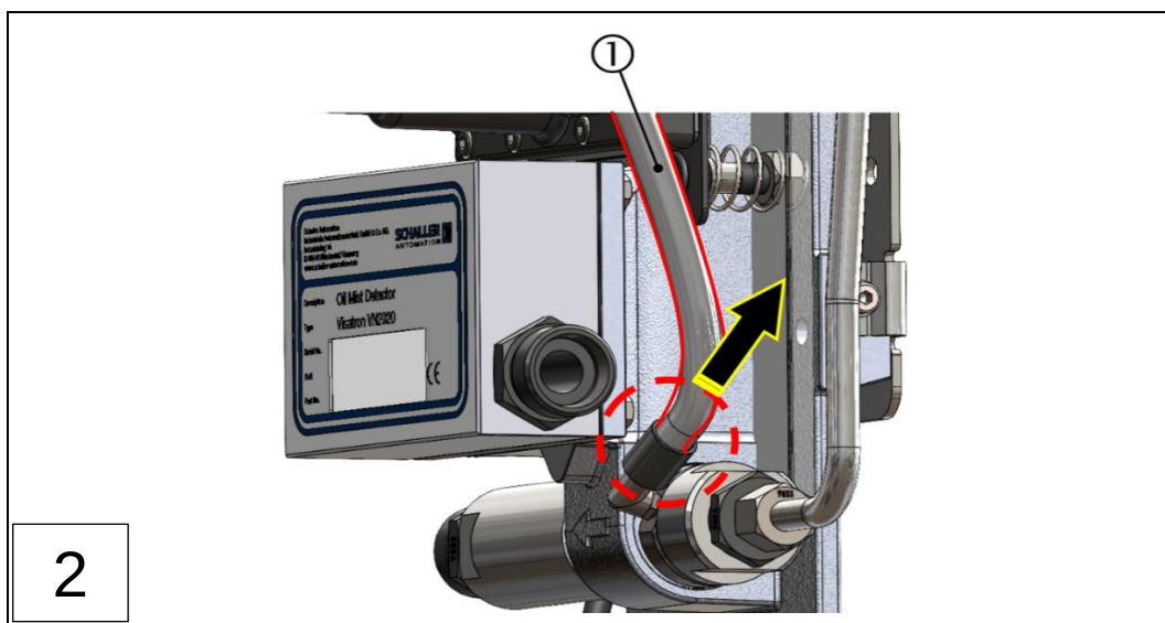
1: Remove the "venturi injector" compressed air hose
