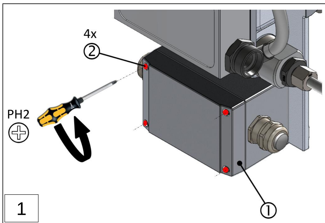
1: Cover, VN2020 terminal box
