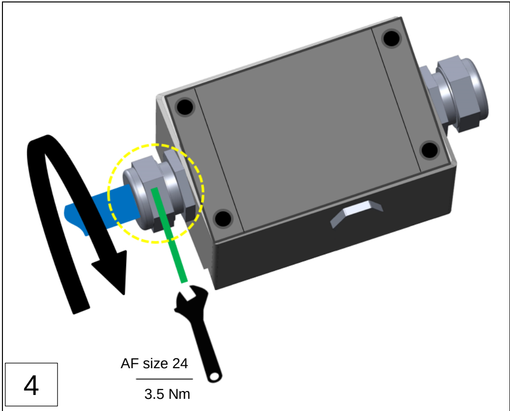
Fig.: 49 : Establishing the power and relay supply (example installation; installation steps 1-4)
