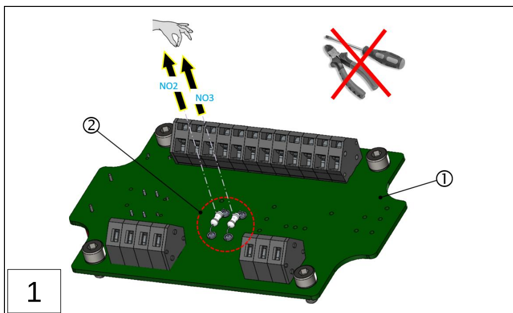
1: Connection board, VN2020 terminal box
