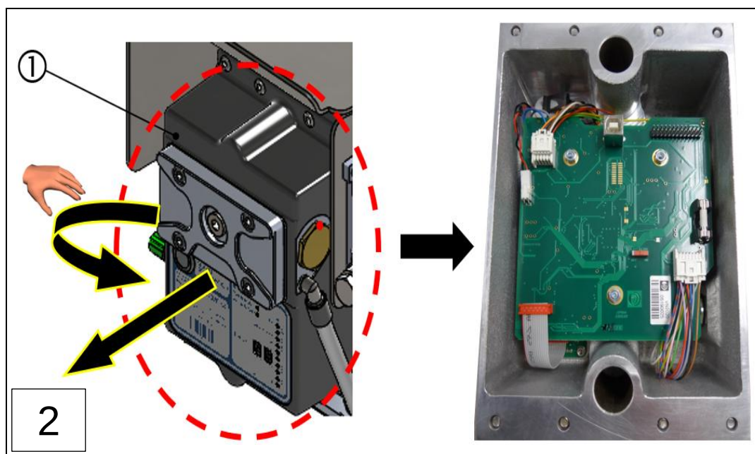
Fig.: 66 : Removing the VN2020 measuring head (installation steps 1-2)
