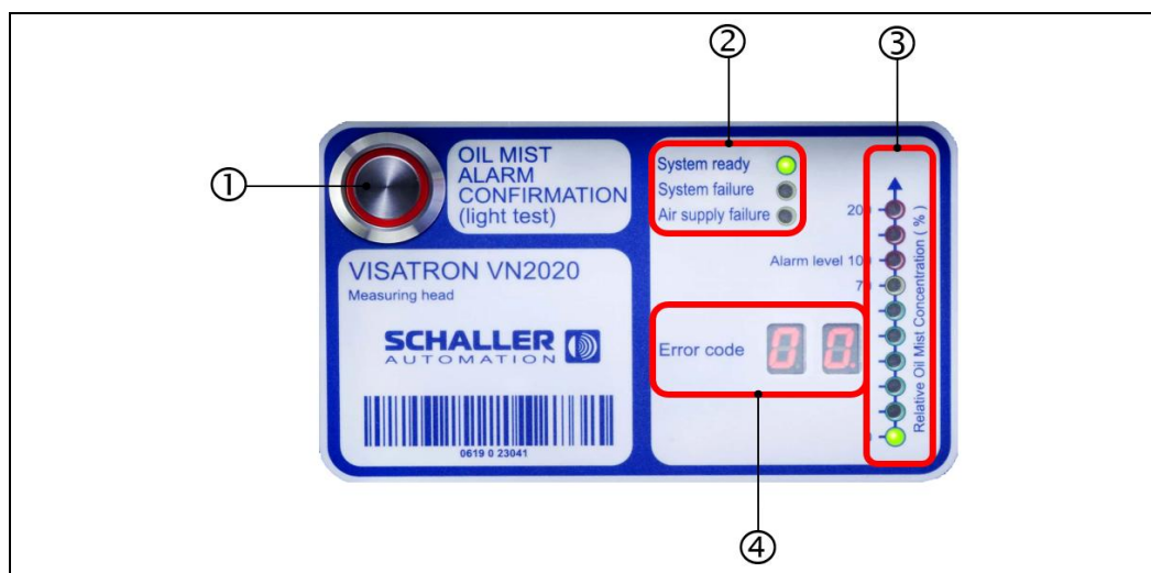
Fig.: 22 : Controls and indicators, VN2020
