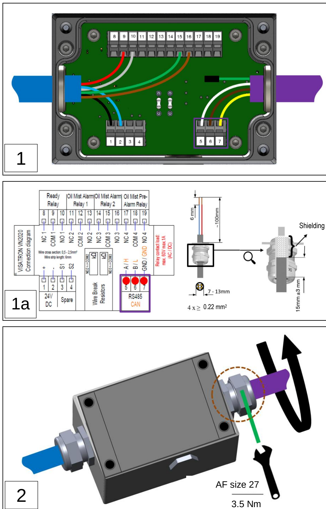
Fig.: 50 : Connecting the Remote Indicator II to terminal box (example inst.; install. steps 1-2)
