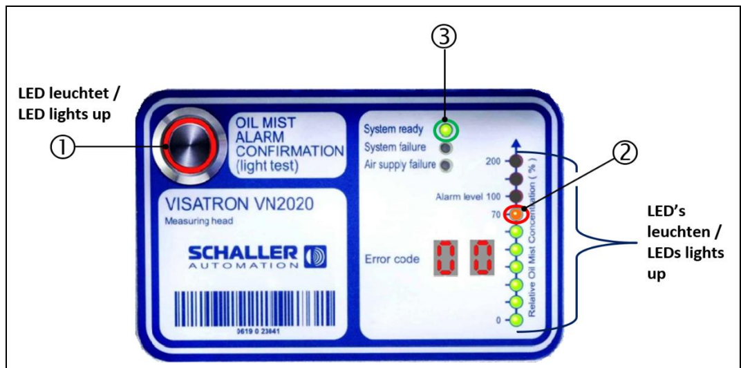
Fig.: 71 : VN2020 measuring head: “Pre-alarm” status indicator at 70% OMC
