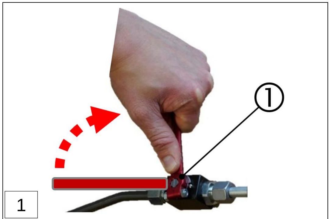
1: Shutoff lever valve (close)
