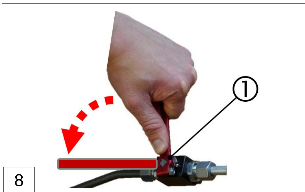
Fig.: 91 : Replacing the filter control valve (steps 1-8)
