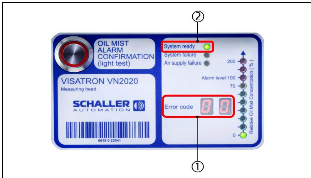
Fig.: 94 : VN2020 measuring head: "System or device error" status indicator
