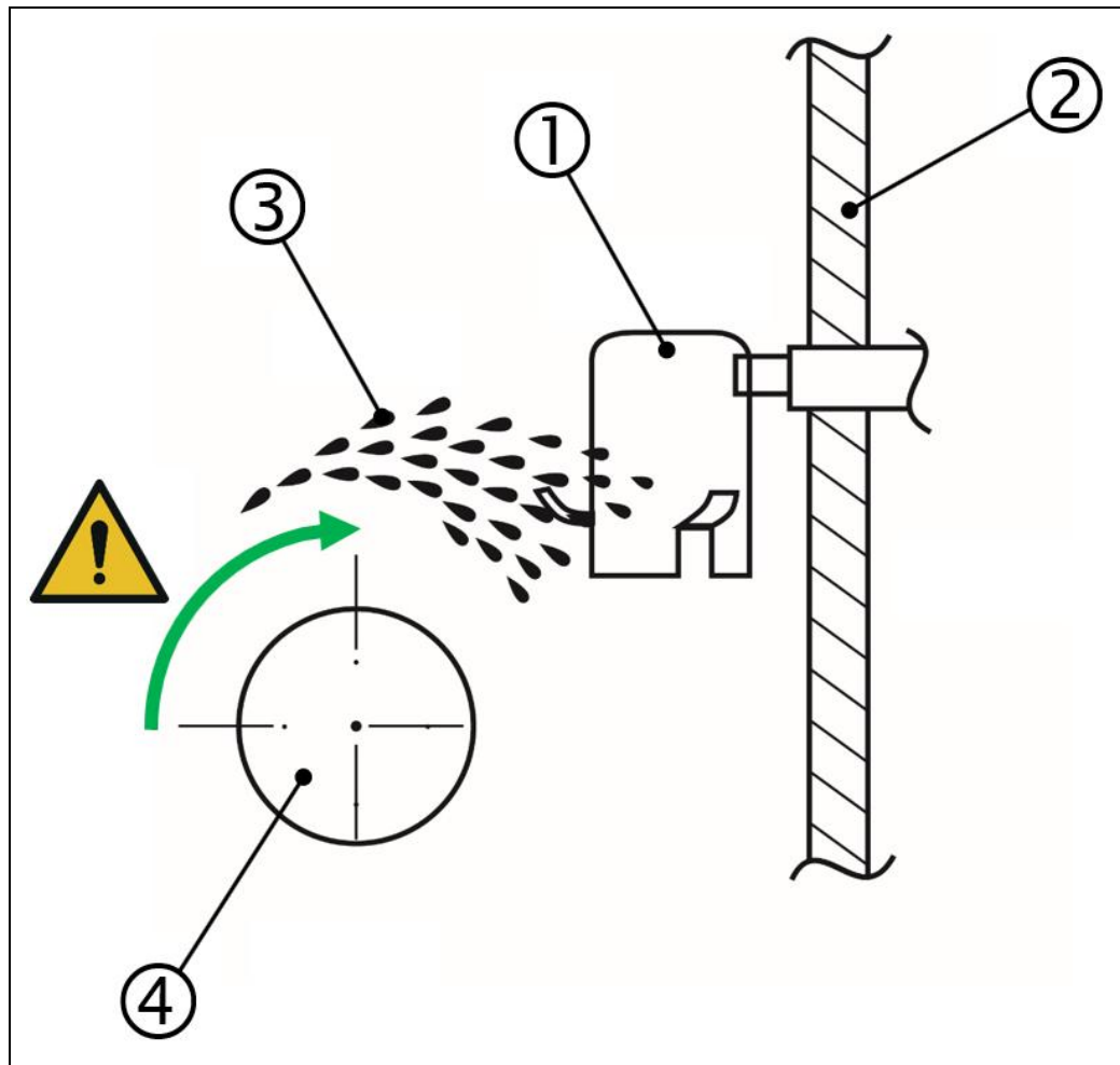
Fig.: 28 : Recommended inst. for the engine wall connection (view from the crankshaft end)
