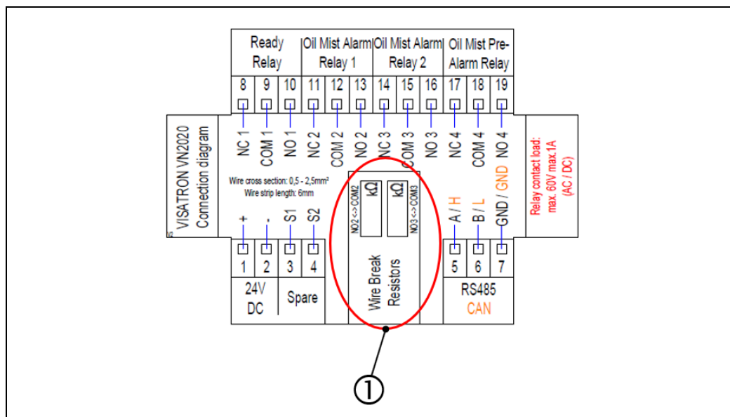
Fig.: 44 : VN2020 terminal box: Configuration of the wire break resistors
