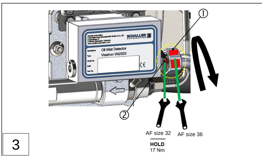
1: "Connecting box" union nut, VN2020
