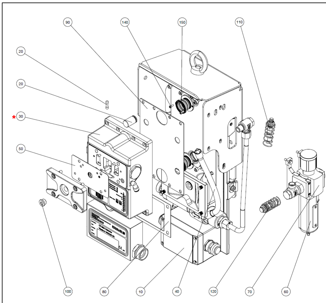
Fig.: 95 : Overview of the positions of spare parts (kept in stock) for the VISATRON® VN2020
