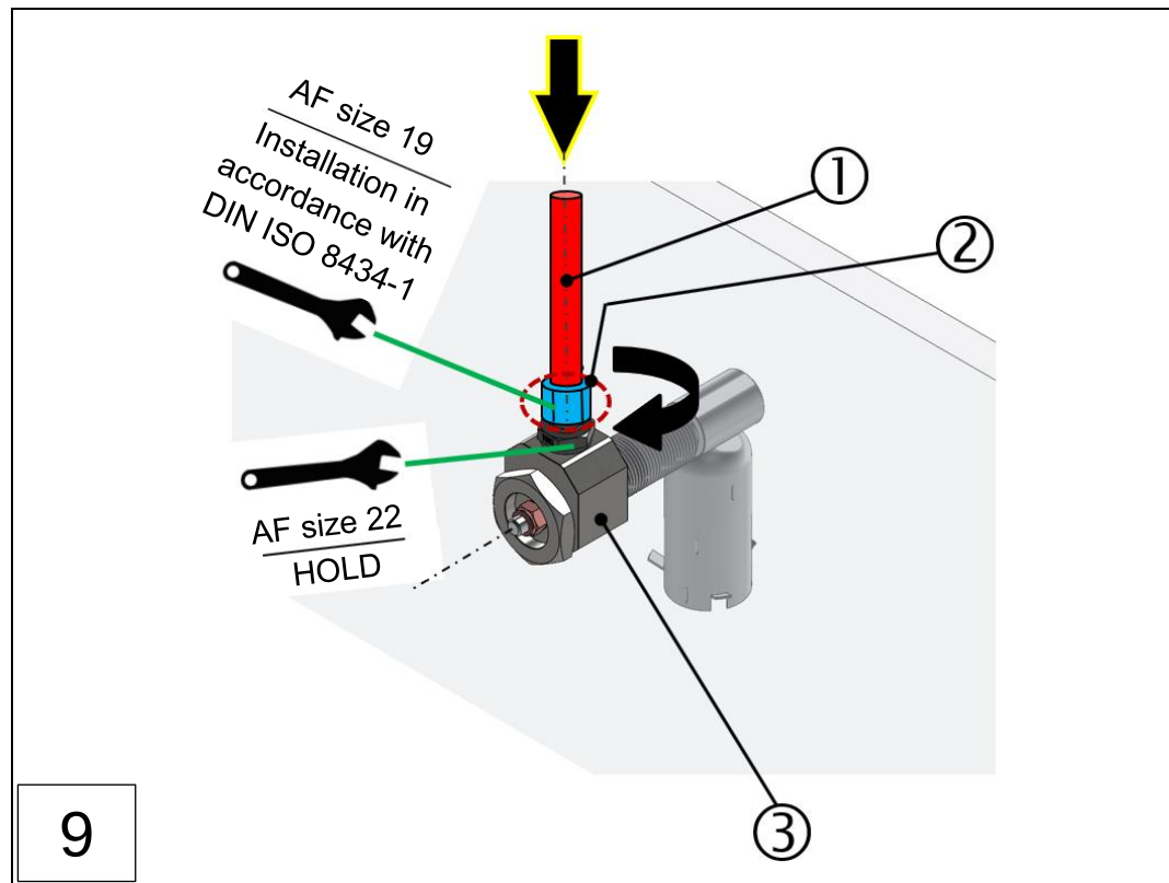
Fig.: 29 : Installing the engine wall connection for the VN2020 (installation steps 1-9)
