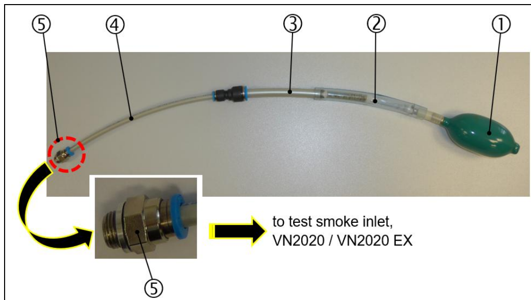
Fig.: 79 : Smoke tube with hand pump (assembled) from Smoke Test Box (151780)
