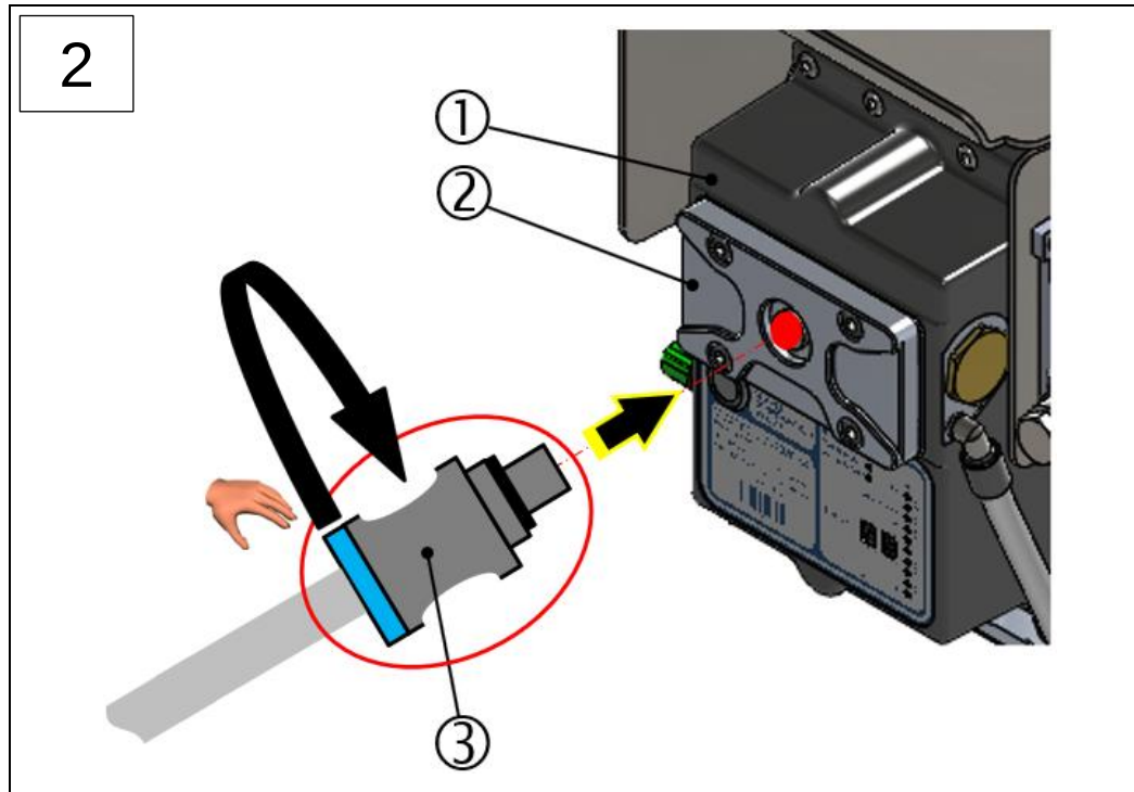
1: Measuring head 3: Push-in fitting with flexible hose
