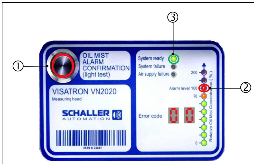
Fig.: 63 : Function test for starting up for the first time, VN2020/VN2020 EX
