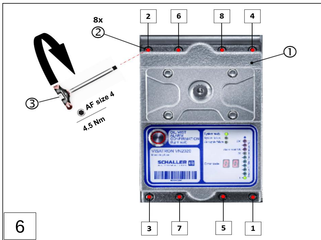
1: VN2020 measuring head 3: Allen key, size 4
